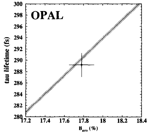
Fig. 3. The OPAL \tau lifetime measurement is plotted against the OPAL measurement of the \tau electronic branching ratio, B_{e\nu\nu} . The straight line shows the prediction assuming lepton universality, and the dotted lines reflect the uncertainty associated with the \tau mass.
