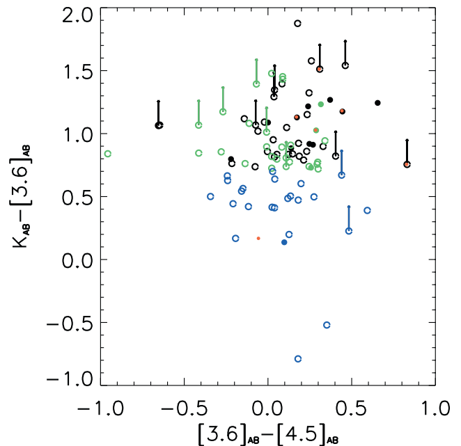
FIG. 1.— K - [3.6] vs. [3.6] - [4.5] color-color diagram for extremely red objects (all magnitudes are AB). The arrows indicate galaxies detected in IRAC channel 1 ( 3.6 \mu\text{m} ) but not detected in the K band (and hence having only a lower limit to their K - [3.6] color). The open and filled blue circles denote EROs selected on the basis of their red R - [3.6] colors. The open and filled green circles denote EROs selected on the basis of their red K - [3.6] colors. The open and filled black circles show EROs in common, i.e., galaxies that would be identified as EROs by either color cut. Galaxies with K - [3.6] > 0 and [3.6] - [4.5] < 0 , i.e., occupying the upper left quadrant, likely lie in the redshift range 0.6 < z < 1.3 . Galaxies with K - [3.6] > 0 and [3.6] - [4.5] > 0 , i.e., occupying the upper right quadrant, likely lie at redshift z > 1.3 . Note that the agreement between the R - [3.6] and K - [3.6] selected samples is best at z > 1.3 . The blue, green and black filled circles, in each case, show galaxies with a MIPS 24 \mu\text{m} detection. Red filled circles denote SCUBA sources (Scott et al. 2002). The two galaxies with color K - [3.6] < 0 are likely dusty local galaxies.
