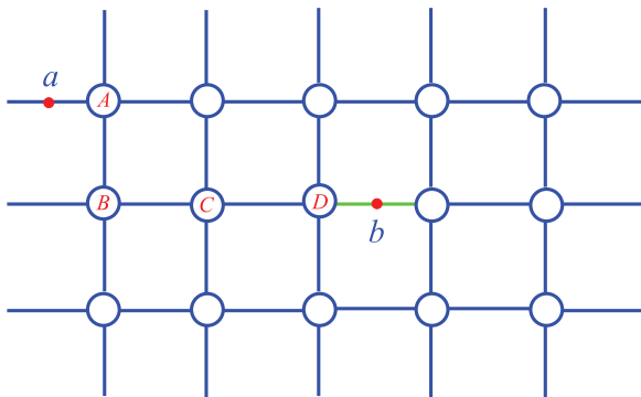
FIG. 7. (Color online) Two-dimensional linear network of resonators, qubits, and qutrits. A short line represents a resonator and each circle represents a coupler qutrit. The two red dots represent qubits a and b . The coupler qutrits A , B , and C are used to transfer information stored in qubit a to the coupler qutrit D . They are also used to transfer information of the coupler qutrit D back to qubit a after a quantum operation is performed on the coupler qutrit D and qubit b , which interact with each other through a resonator (i.e., the green short line).
