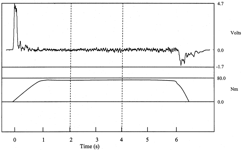
Figure 2 — Example of the raw MMG signal from the biceps brachii and the isometric torque production curve. The portions of the MMG and torque signals between the dashed vertical lines were selected for analysis.
