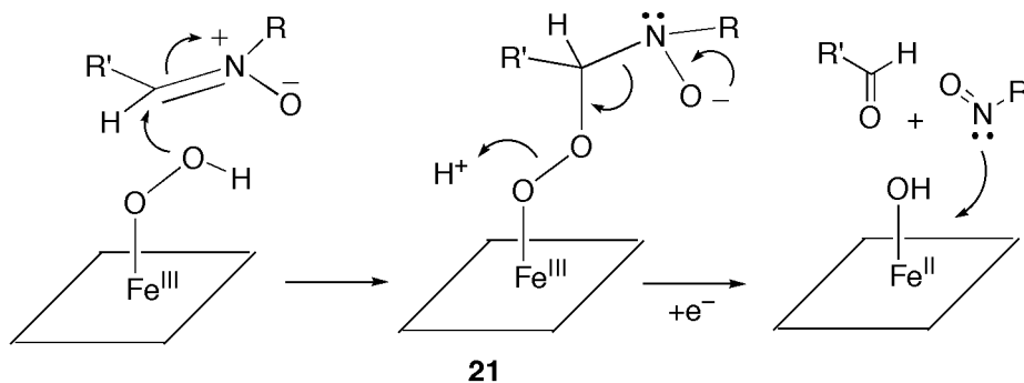
Figure 9. Proposed mechanism for oxidation of nitron 5 to a nitroso intermediate for oxime formation and MIC formation.
