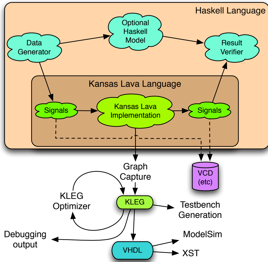
Figure 3.1. KansasLava Architecture
