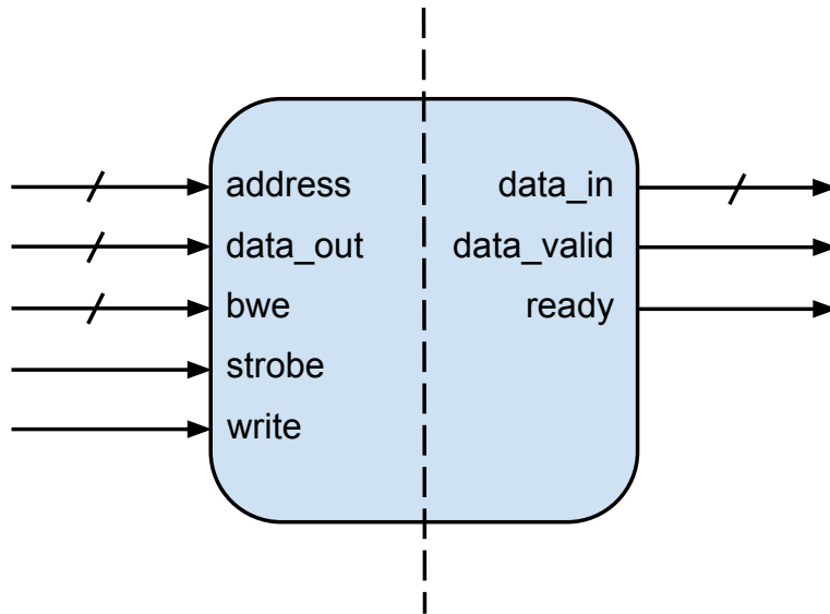
Figure 6.1. Annapolis Wildstar 5 DRAM Interface
