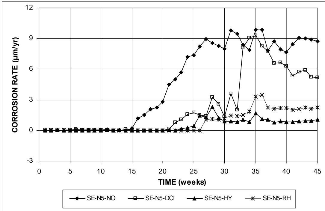
Figure 3.24 – Southern Exposure Test. Average corrosion rates for specimens with conventional steel and different inhibitors.
