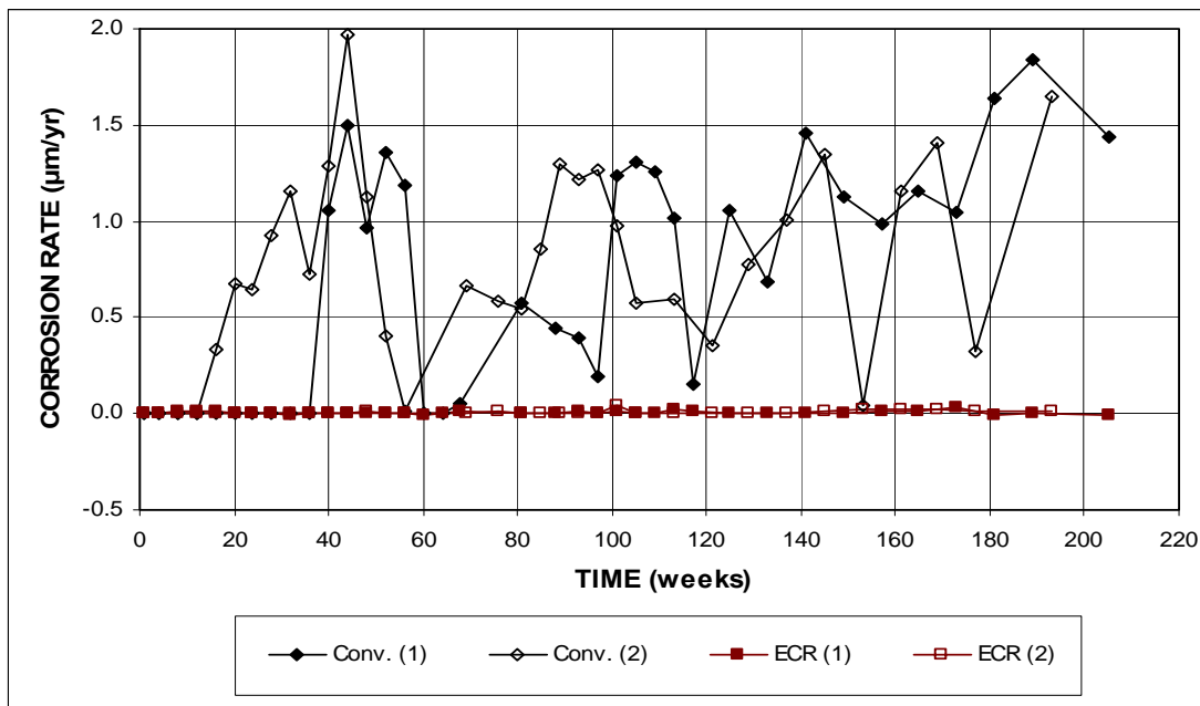
Figure 3.48a – Field Test. Average corrosion rates for specimens with conventional steel and ECR, with cracks (ECR with 16 holes through the epoxy).
