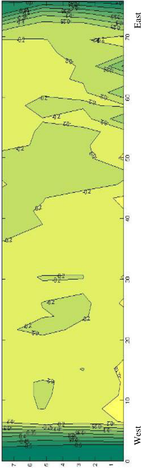
Figure C.7 – Corrosion potential map for the Doniphan County Bridge (October 12, 2007)
