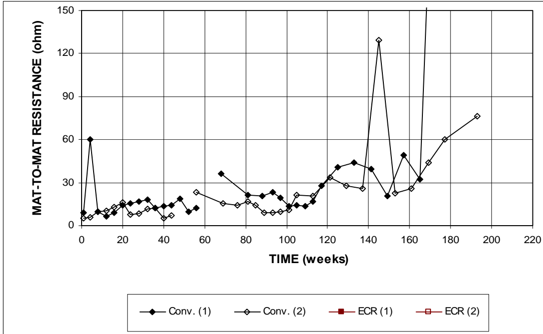
Figure 3.47b – Field Test. Average mat-to-mat resistances for specimens with conventional steel and ECR, without cracks (ECR with 16 holes through the epoxy). (Different scale)
