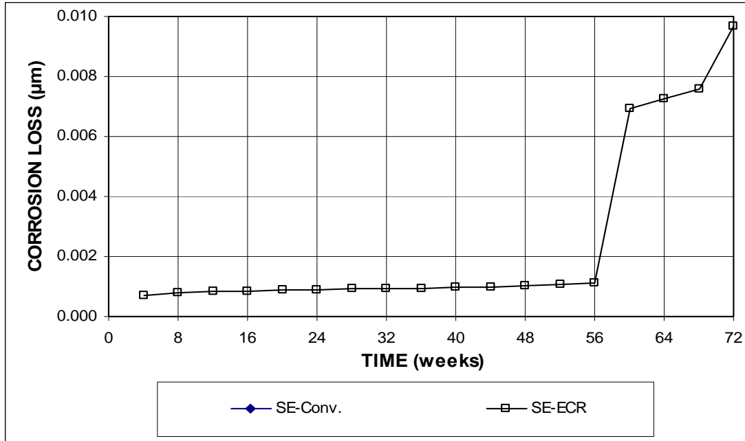
Figure 3.118b – Microcell corrosion losses from LPR method for the top mats in specimens with conventional steel and ECR in the Southern Exposure test (ECR have four holes through the epoxy). (Different scale)
