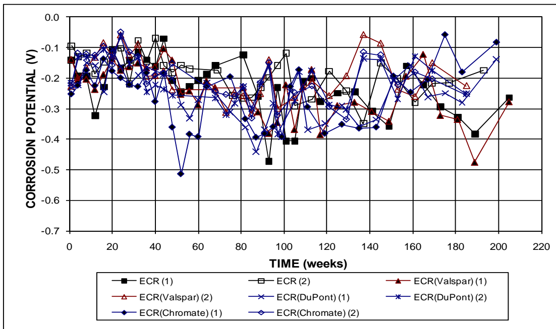
Figure 3.88b – Field Test. Average bottom mat corrosion potentials with respect to a copper-copper sulfate electrode for specimens with ECR and ECR with increased adhesion, with cracks (ECR with 16 holes through the epoxy).
