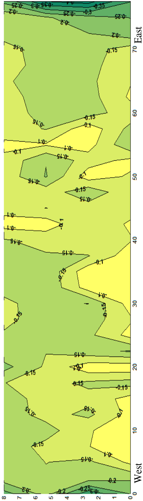
Figure C.3 – Corrosion potential map for the Doniphan County Bridge (October 14, 2005)
