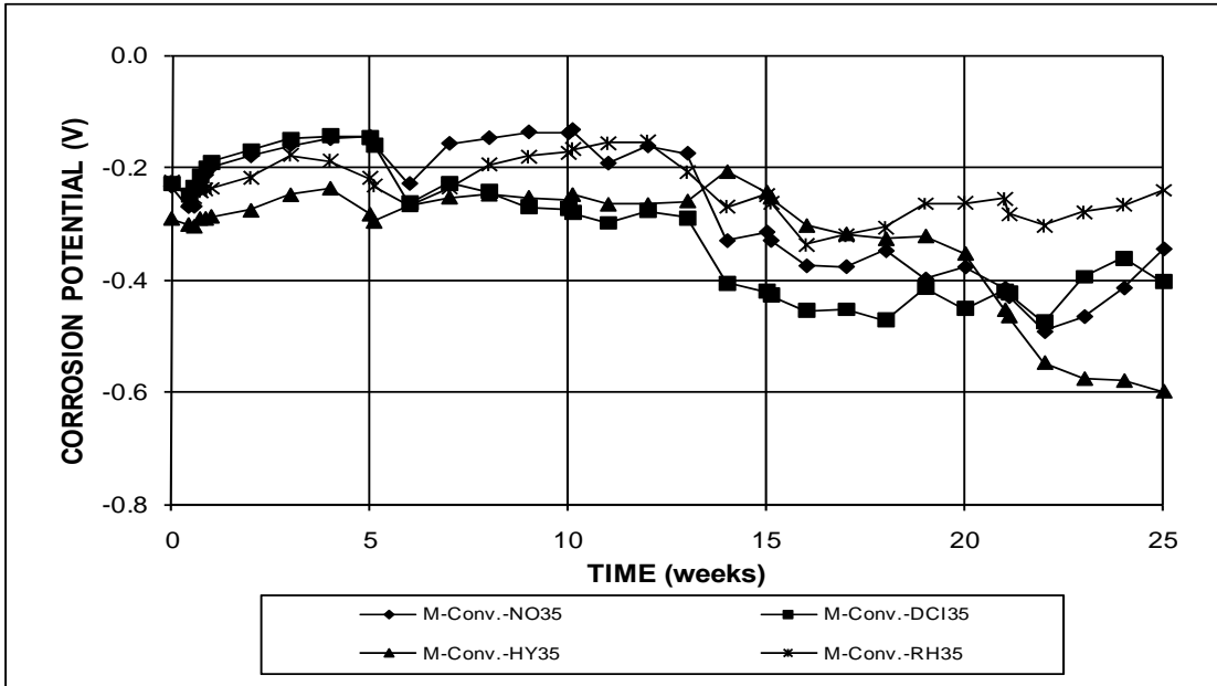
Figure 3.4a – Macrocell Test. Average anode corrosion potentials with respect to a saturated calomel electrode for specimens with conventional steel and different inhibitors, w/c = 0.35 . (Based on average of six specimens before week 20 and three specimens after, except two specimens are used for Hycrete after week 20)
