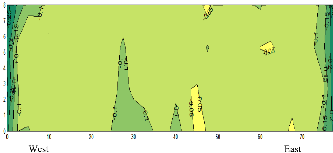
Figure 3.110 – Corrosion potential map for the Doniphan County Bridge (1 st survey, September 17, 2004).
