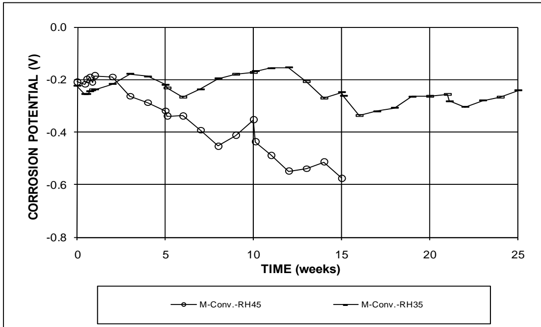
Figure 3.12a – Macrocell Test. Average anode corrosion potentials with respect to a saturated calomel electrode for specimens with conventional steel and specimens with different water-cement ratios, Rheocrete inhibitor.
