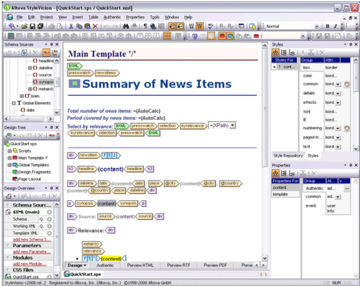
Figure 10: Altova StyleVision® 2008
