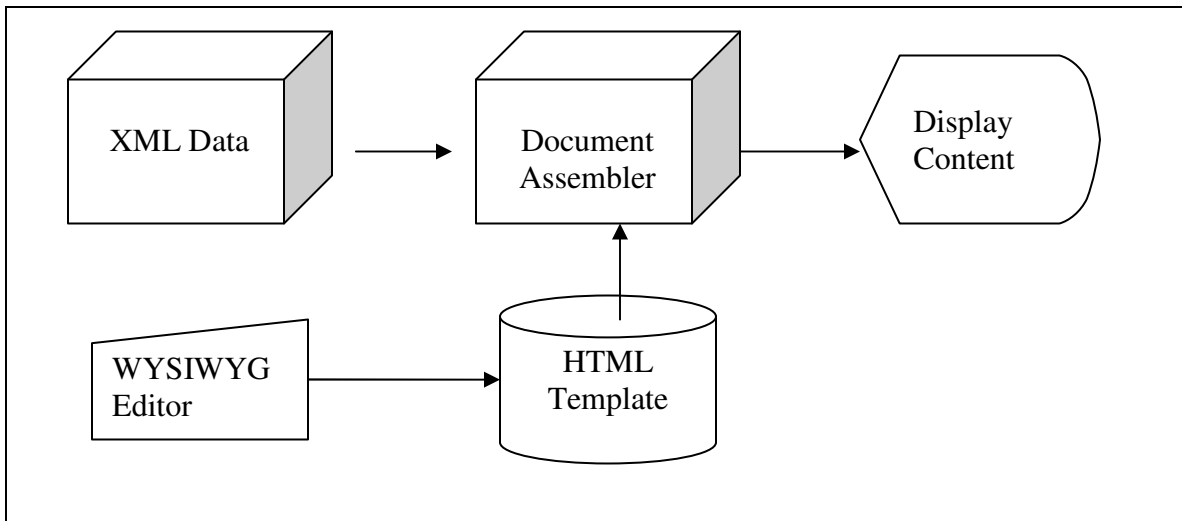
Figure 16: Process flow diagram of the proposed XML data presentation system
