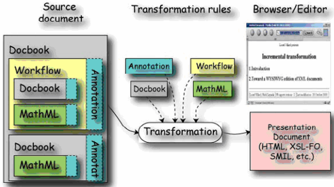
Figure 3: Incremental Transformation (Villard and Layaïda 2001)
