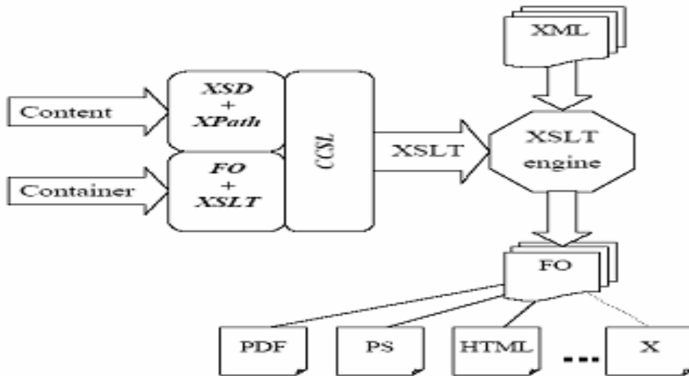
Figure 7: CCSL Transformation (Canfora and Cerulo 2002)
