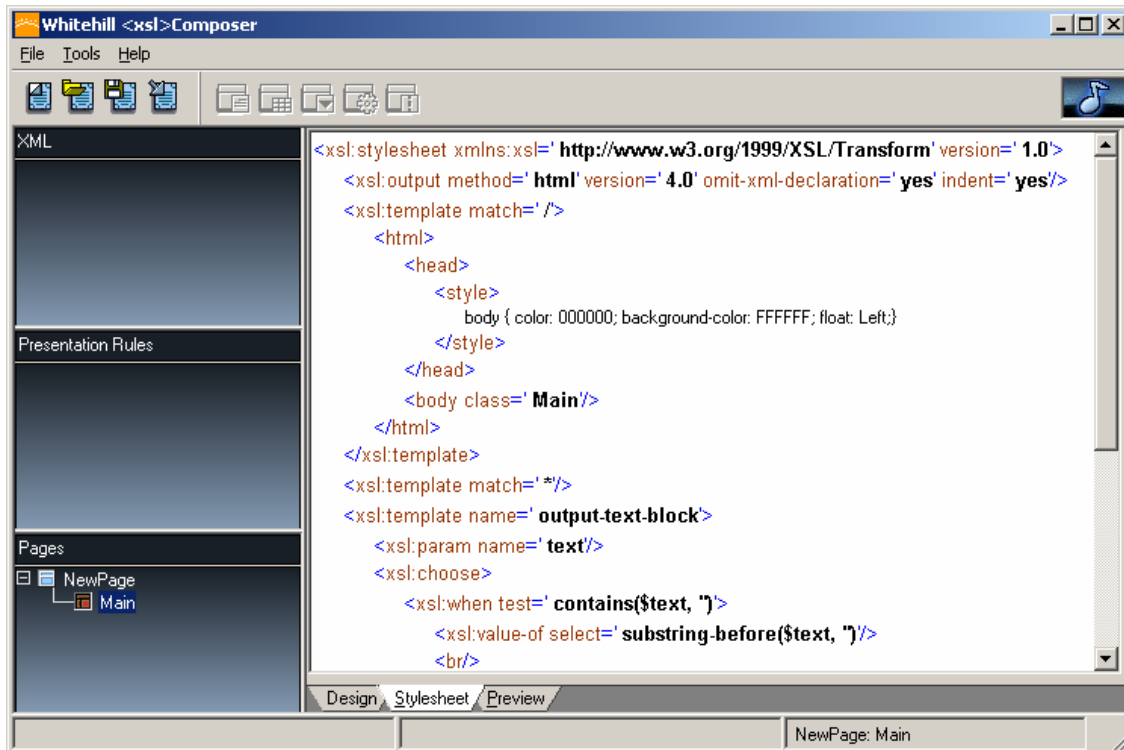
Figure 5: Whitehill XSLComposer
