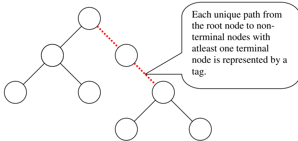
Figure 11: Example of a unique path represented by a tag
