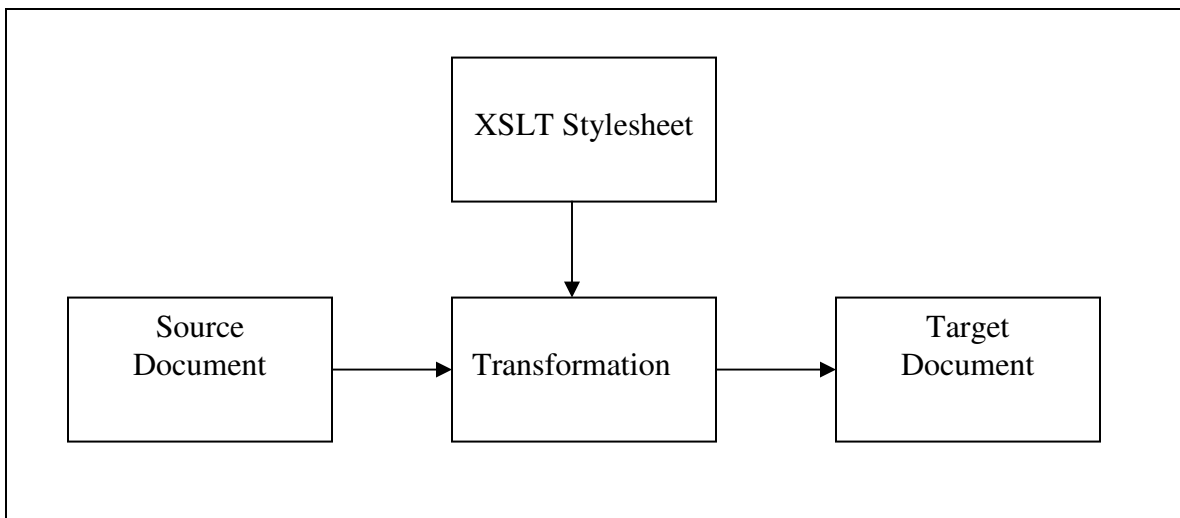
Figure 2: XSLT Transformation
