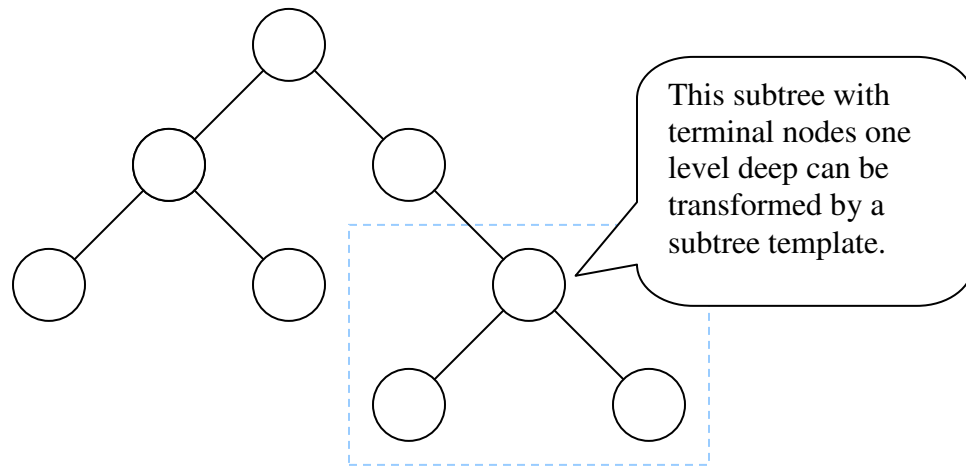
Figure 14: Subtrees transformed by subtree templates
