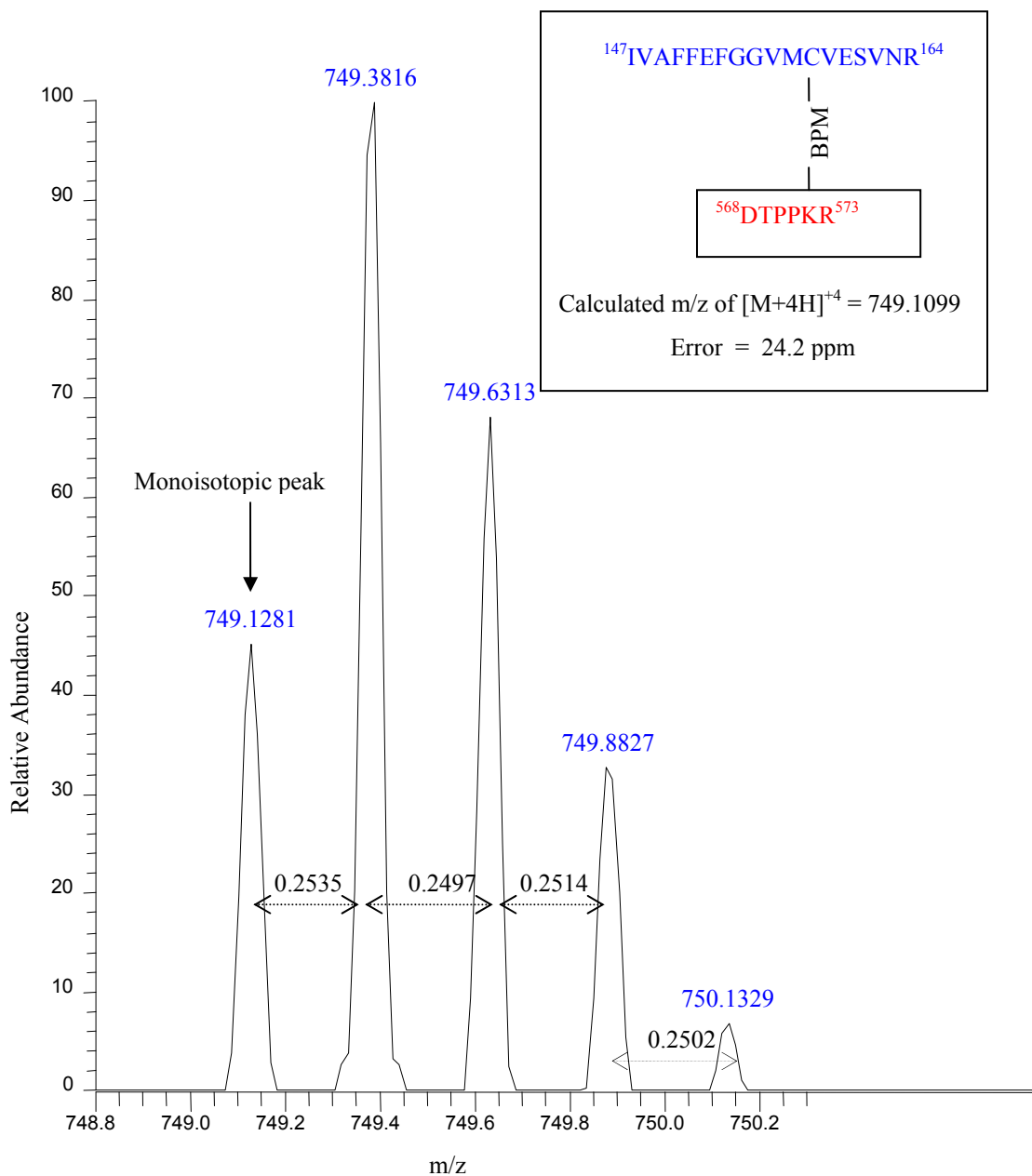
FIGURE 2.19: Mass Spectrum of [\text{M}+4\text{H}]^{+4} of the cross-linked SERCA-Bcl-2Δ21 dipeptide: The isotopic peak distribution of MS1 of quadruply charged ion is shown. The spacing between peaks are shown confirming the +4 charge state. In-set shows the cross-linked dipeptide, peptide of SERCA in red and peptide of Bcl-2Δ21 in blue.
