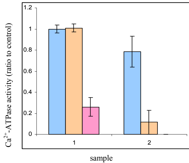
FIGURE 4.1: Effect of W188A mutant of Bcl-2Δ21 on Ca 2+ -ATPase activity of SERCA: (●)-SR alone; (○)-SR mixed with wild type Bcl-2Δ21; (●)-SR mixed with W188A mutant of Bcl-2Δ21; 1-before incubation at 37 °C; 2-after 1h of incubation at 37 °C.
