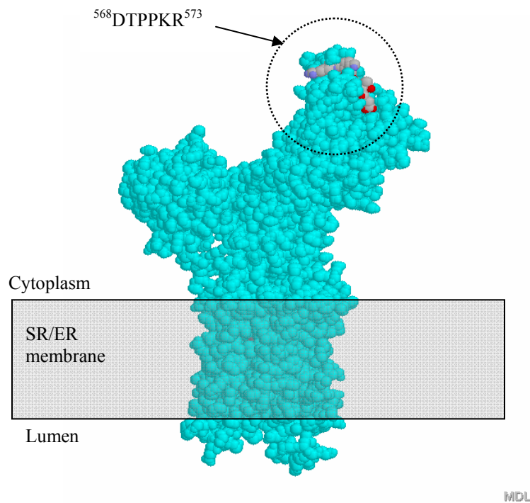
FIGURE 2.22: The 3-D structure of SERCA showing the peptide cross-linked to Bcl-2 \Delta 21: ^{568}\text{DTPPKR}^{573} peptide of SERCA located in the ATP binding domain is circled. The structure of SERCA is from protein data bank (PDB code 1SU4).
