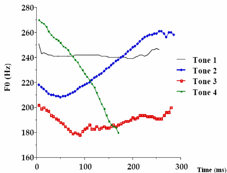
Figure 1. F 0 contours for the four Mandarin tones, each combined with the syllable ma produced by a female native speaker (from Moore and Jongman, 1997).
