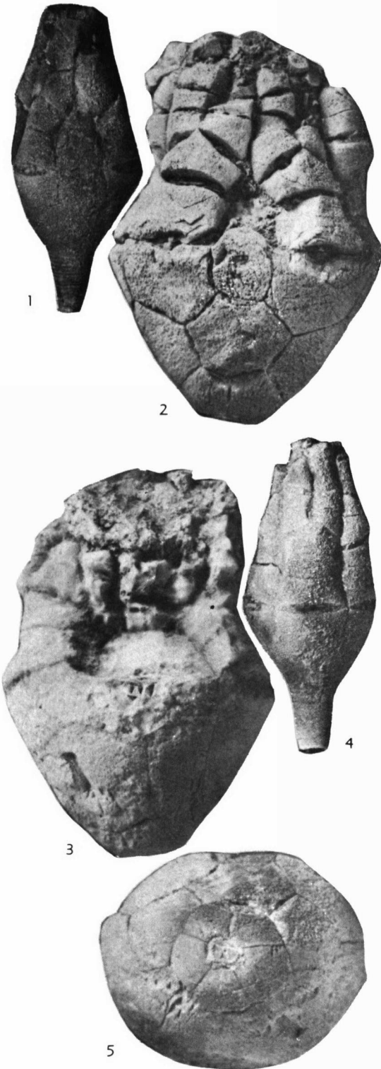
FIG. 10.—1,4. Armenocrinus watersi STRIMPLE & HORO-
