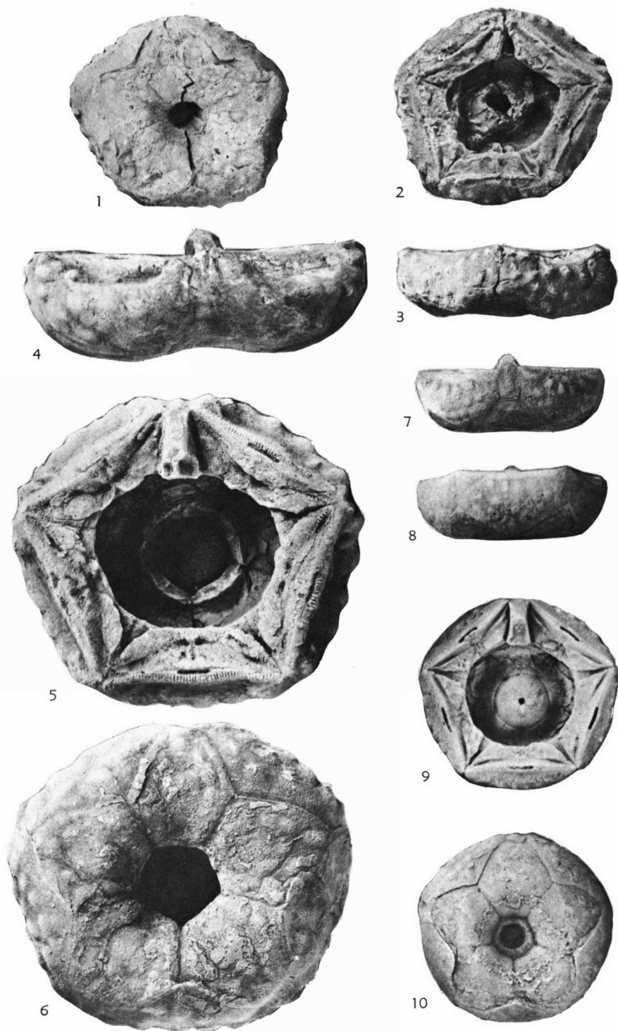
FIG. 2. Atokacrinus and Diphuicrinus from Oklahoma. (Continued on facing page.)
