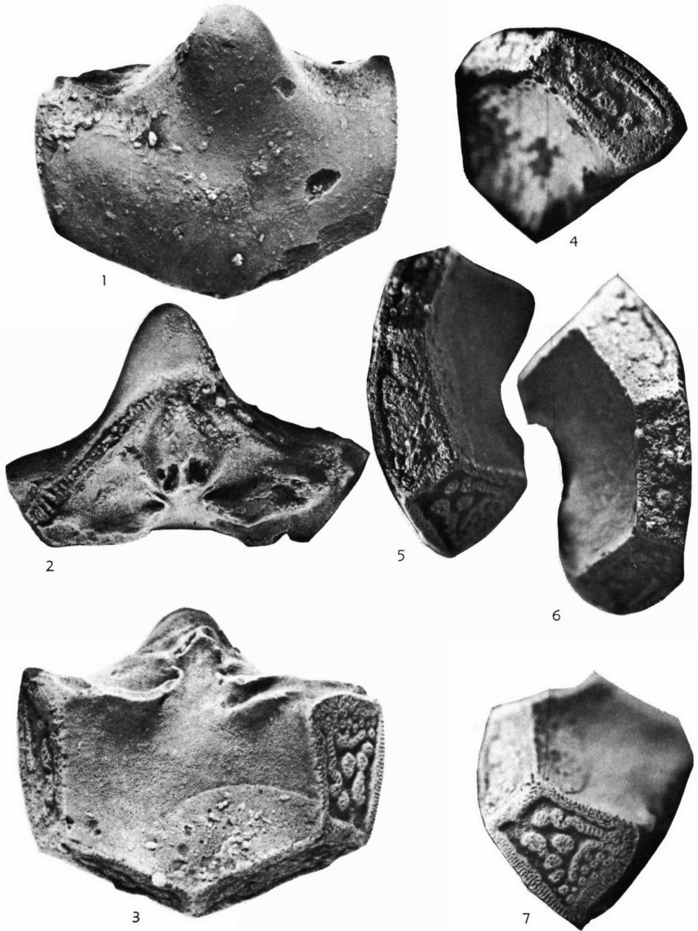
FIG. 7,1-7. Delocrinus subhemisphericus MOORE & PLUMMER from the Lane Shale (Upper Pennsylvanian) of Kansas City. A dual plate consisting of both a radial and primibrach I viewed from front, summit, interior, right lateral side, right proximal side, left proximal side, and left lateral side, \times 6.5 .
