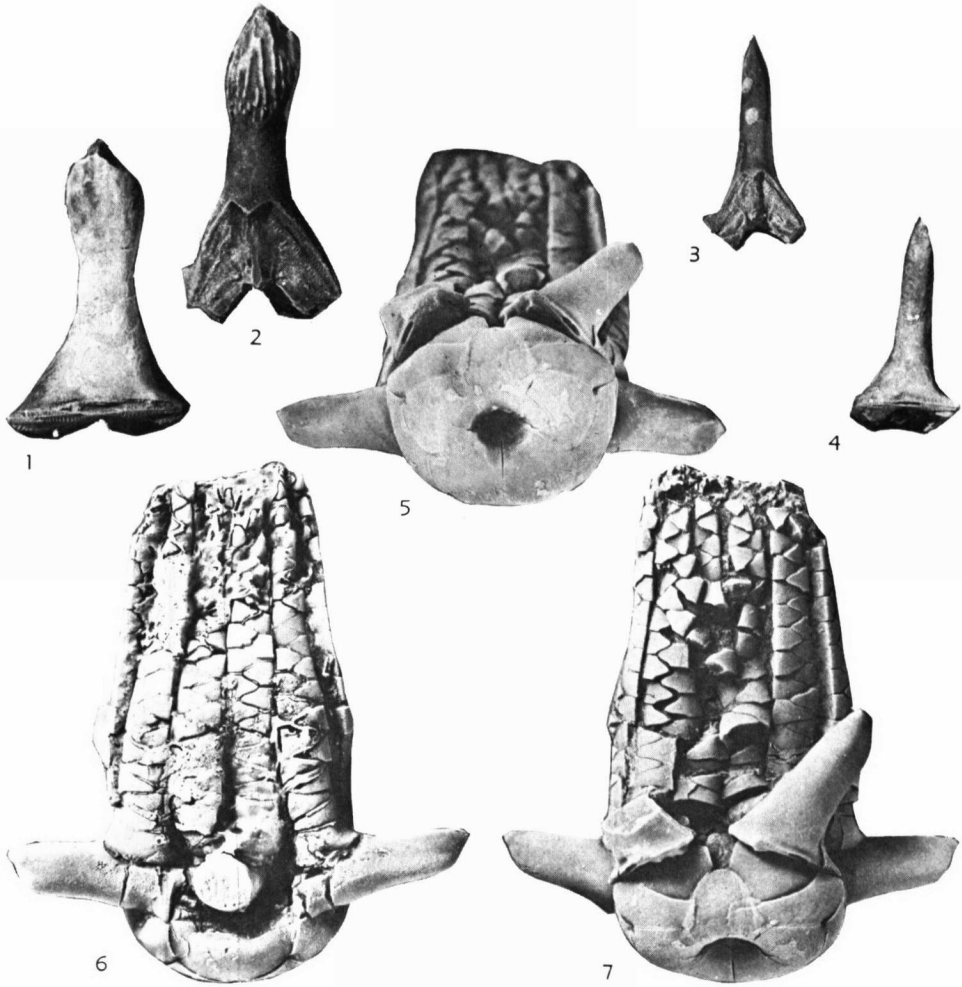
FIG. 8. Delocrinus and Endelocrinus from the Lane Shale (Upper Pennsylvanian) at Kansas City.
