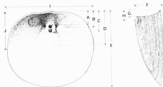
FIG. 5. Diagrammatic representation of the location of measurements on the ventral valve of Quadrisonia minor .
