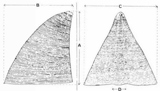
FIG. 2. Diagrammatic representation of the location of measurements on the ventral valve of Dactylotreta redunca .
