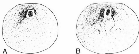
FIG. 4. Variation in form of apical process of Quadrisonia minor .
