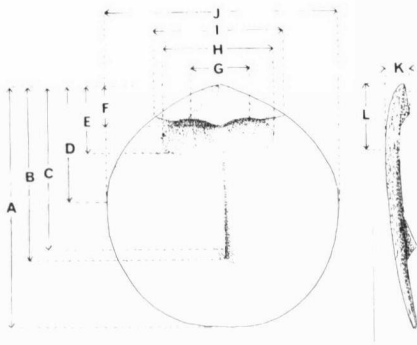
FIG. 3. Diagrammatic representation of the location of measurements on the dorsal valve of Dactylotreta redunca .
