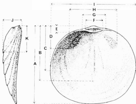
FIG. 8. Diagrammatic representation of the location of measurements on the dorsal valve of Anabolotreta tegula .
