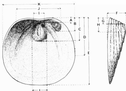
FIG. 7. Diagrammatic representation of the location of measurements on the ventral valve of Anabolotreta tegula .
