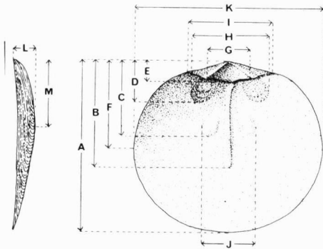
FIG. 6. Diagrammatic representation of the location of measurements on the dorsal valve of Quadrisonia minor .
