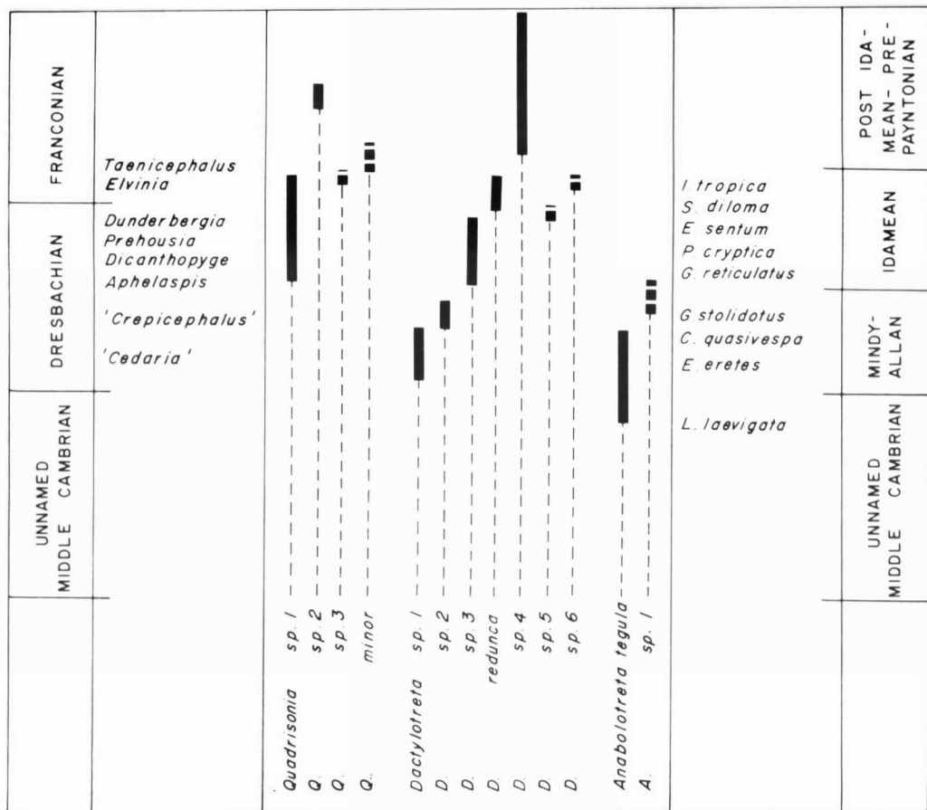
FIG. 1. Stratigraphic ranges of known species of Quadrisonia , Dactylotreta , and Anabolotreta . Approximate correlation of North American stages and zones (on the left) with those of Australia (on the right) based on Henderson (1976). Australian species ranges in solid black, North American species in heavy broken line.
