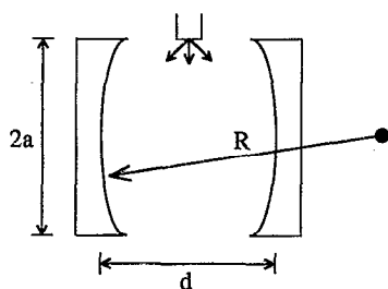
FIG. 1. Fabry-Perot cavity parameters.
