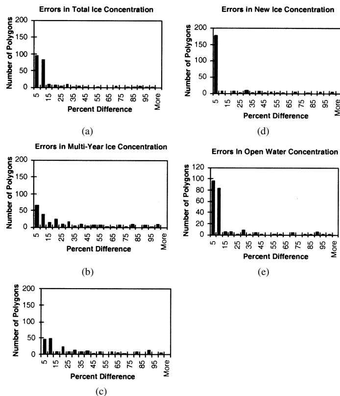
Fig. 4. Distributions of ice concentration differences (absolute value) for (a) total ice concentration, (b) multiyear ice, (c) first-year ice, (d) new ice, and (e) open water.
