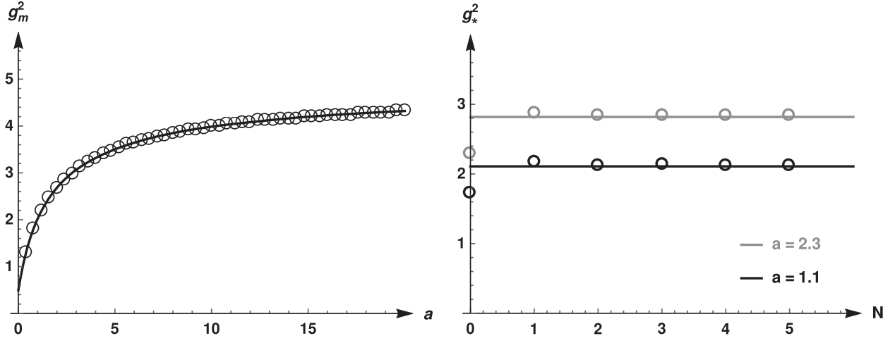
FIG. 2. Left panel: Fixed point values g_m^2 as provided by shooting from the origin for different a . The solid line is a fit; for the interpolating function; see Eq. (62). Right panel: Comparison of shooting from the origin and polynomial truncation. The solid line is located at g_m^2(a) as obtained from the interpolating function. The g_*^2(a, N) due to polynomial truncation of order N converge to g_m^2(a) .
