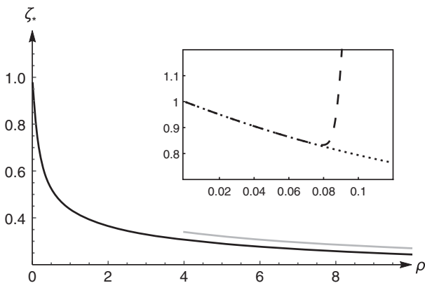
FIG. 3. The critical Kähler metric for a = 1.75 . The solid black line is produced by pseudospectral methods, while the solid gray line shows a \rho^{-1/4} decay. Inset: The pseudospectral solution (dotted line) is compared to the one obtained by shooting from the origin (dashed line) with g_*^2 = 2.576 corresponding to a maximum of \rho_s as in Fig. 1.
