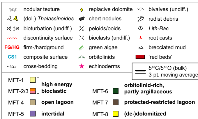
Fig. 4. Lithostratigraphy including identified microfacies types (MFT-1 to MFT-8) and main fossil constituents and carbon and oxygen isotope stratigraphy of the Jabal Madar section, complemented with data from Pittet et al. (2002) and Sattler et al. (2005). Sequence stratigraphic interpretation after Pittet et al. (2002). At first glance, the low covariance between \delta^{13}\text{C} and \delta^{18}\text{O} values ( r^2 = 0.12 ) of all analysed bulk carbonate samples (0 to 74 m) points to the absence of major diagenetic alteration of isotope ratios. Splitting the data into two stratigraphic groups (A/B), however, provides r^2 -values that are indicative of a moderate (0 to 48.8 m: r^2 = 0.41 ) to strong correlation (49.6 to 74 m: r^2 = 0.65 ) of carbon and oxygen isotope values.
