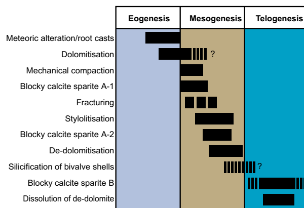
Fig. 8. Paragenetic sequence of different diagenetic processes and products as recorded by Barremian–Aptian shallow-water limestones at the Jabal Madar dome.
