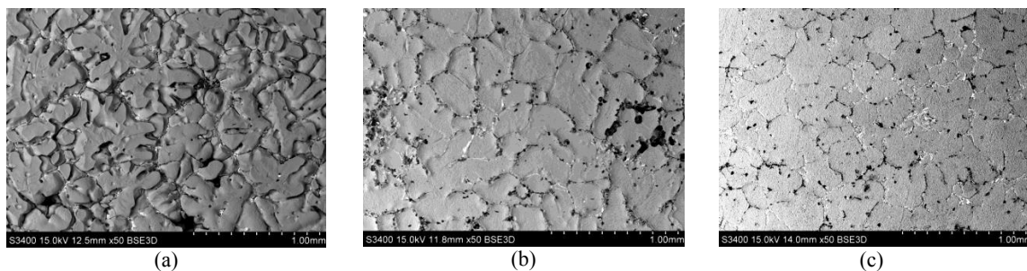
Fig. 1: The structure of specimens solidified in natural conditions (a), stirred with continuously applied AMF (b) and pulsed resonant AMF (c). Magnification is \times 50 .
