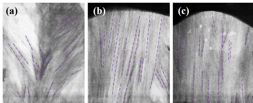
Fig. 3: The visualized macro-crystalloid structure formed in natural conditions (a), stirred with resonant pulsed TMF (b) and with steadily applied TMF (c). Images demonstrate ingots on 150 th -minute from the solidification begin.
