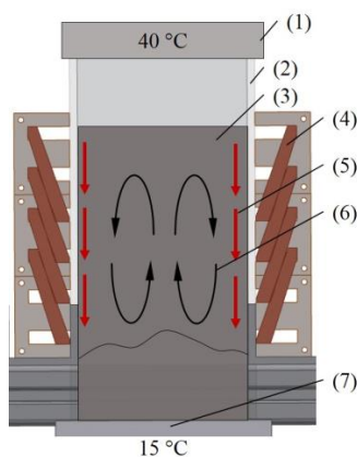
Fig. 2: The experimental system, used for visualization of EM-stirred solidifying pure gallium by means of neutron radiography.
