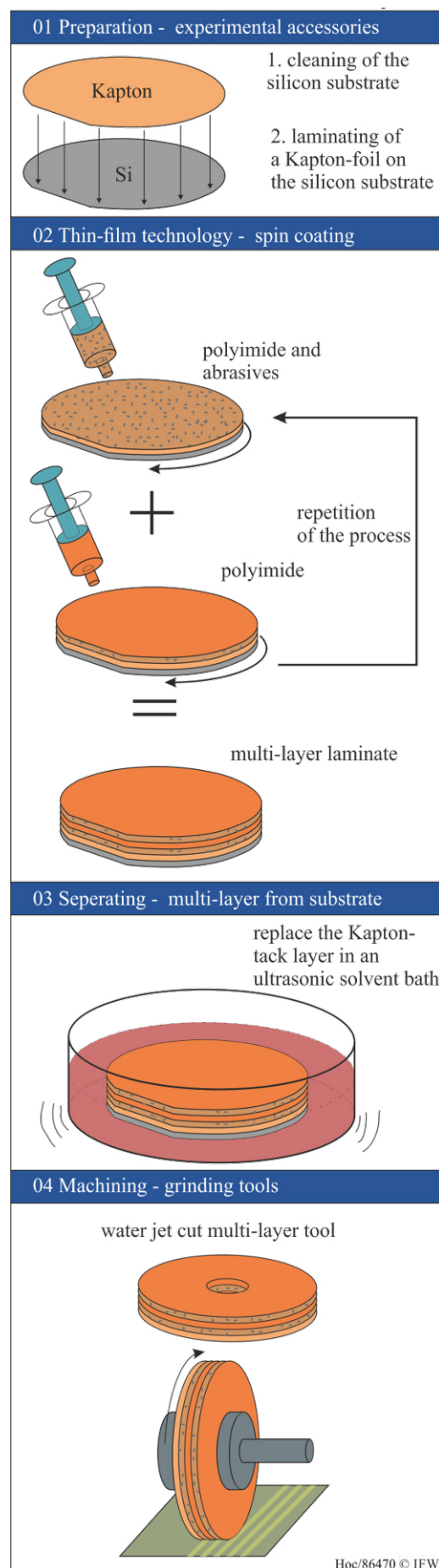
Fig. 1. Manufacturing process of multi-layer tools
