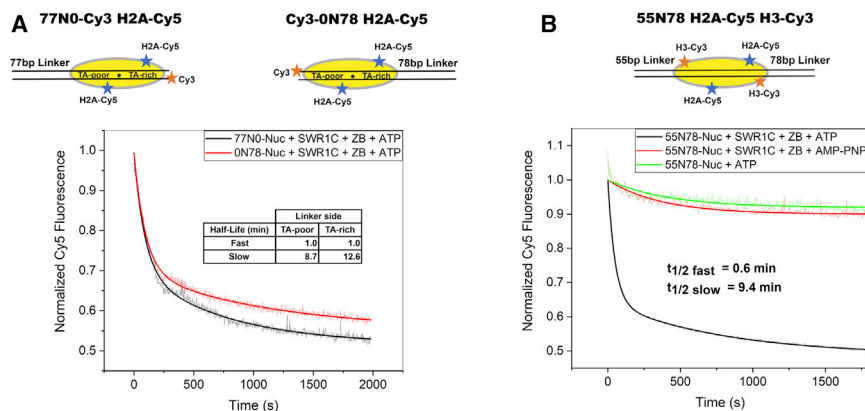
Figure 6. Nucleosome Determinants of Asymmetric Dimer Exchange
