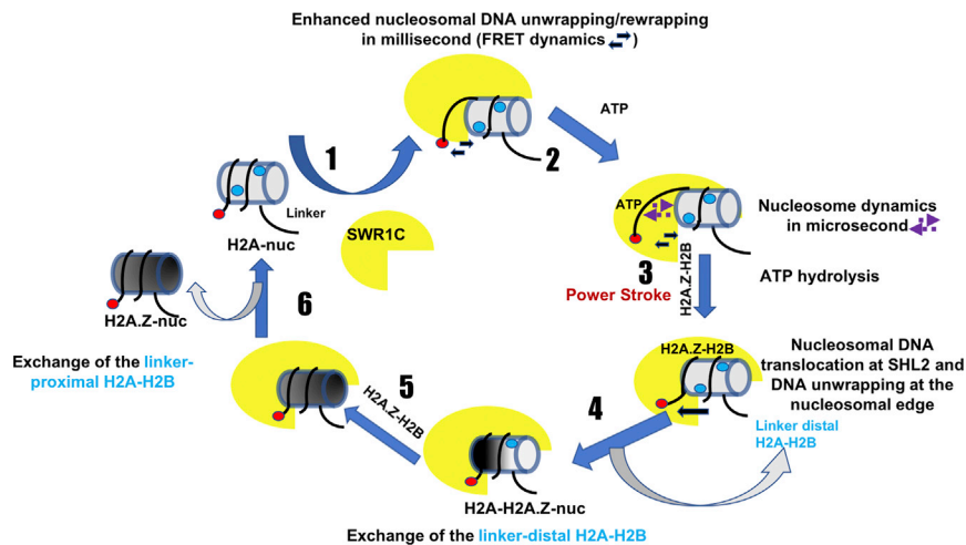
Figure 7. Kinetic Model of the SWR1C-Catalyzed Histone Dimer Exchange Reaction
