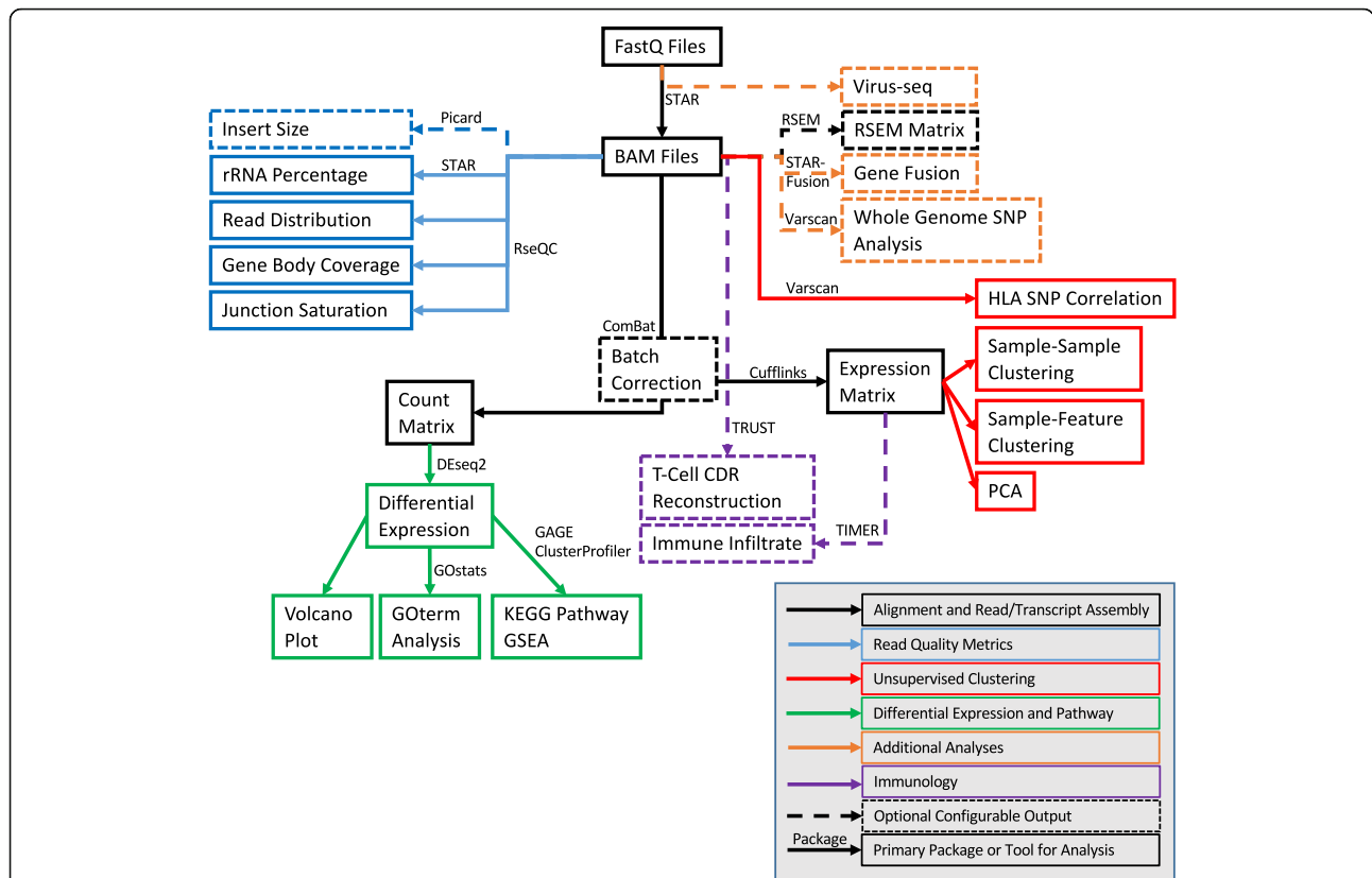
Fig. 1 Overview of the full workflow performed by VIPER (Visualization Pipeline for RNAseq analysis). The different segments of the pipeline are broken down by color. The core of the pipeline is the read alignment performed by STAR that outputs alignment (bam) files. Gene expression is quantitated with Cufflinks for unsupervised analysis (clustering and PCA). STAR also generates a count matrix used for supervised analysis (differential expression with DESeq2). When a publically available analysis tool is used for a particular step, the name of the tool is identified above the arrow leading to the resulting output (boxed). When there is no tool indicated next to an arrow, the analysis step was performed with custom R code. Conditional/optional analyses are denoted with a hashed arrow and outlining box and represent the most distinguishing functionality for VIPER
