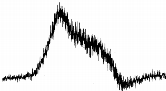
Fig. 2. ^{13}\text{C} -NMR solid state spectrum of a sample of anthracite coal, PSOC No. 80 over a 10,000 Hz sweepwidth (665 ppm), peaks are approx. 140 ppm and -7 ppm from TMS.
