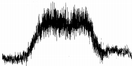
Fig. 1. ^{13}\text{C} -NMR solid state spectrum of a sample of subbituminous coal, group B PSOC No. 240 over a 10,000 Hz sweepwidth (665 ppm), peaks are approx. 140 ppm and -7 ppm from TMS.
