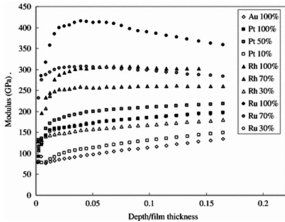
Figure 7. Modulus of thicker films (~1500 nm thickness).
