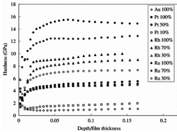
Figure 6. Hardness of thicker films (~1500 nm thickness).
