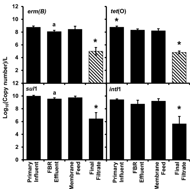
Fig. 2 Abundance of antibiotic resistance genes erm(B) , tet(O) , and sul1 and the class 1 associated integrase gene ( int11 ) per liter from the AnMBR. Bars represent the average value and error bars represent the standard deviation from four sampling events. Striped bars represent reported results equivalent to the detection limit because only one or two samples out of four were quantifiable. The asterisk (*) denotes significant difference from all other sample locations, the (a) denotes significant difference compared to primary sample.
