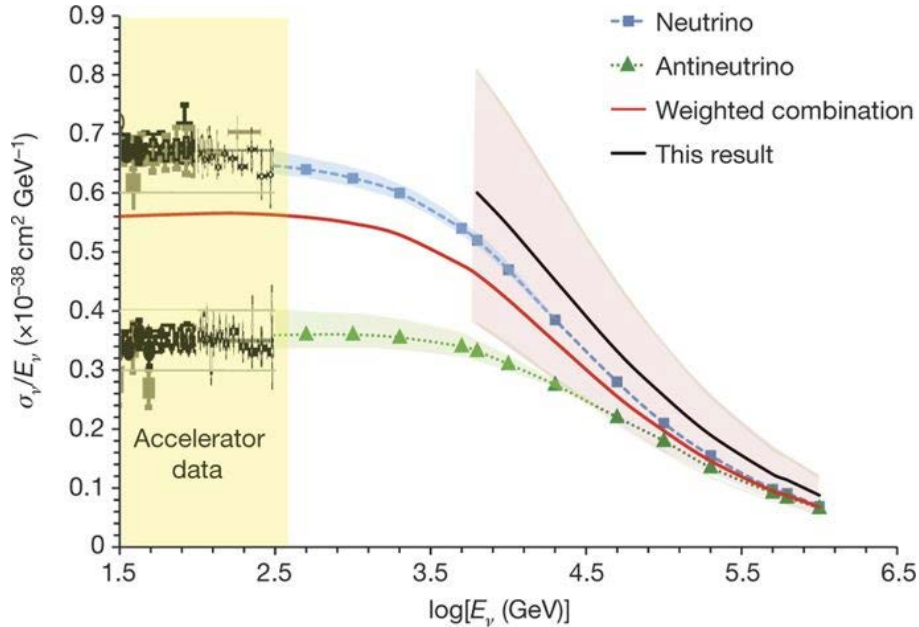
Figure 1: Neutrino cross-section measurements.
