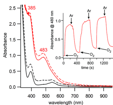
Fig. 7 UV-visible spectral changes during the reaction of complex 4 with O 2 at -70 °C in CH 2 Cl 2 . Treatment of the starting complex (black solid line) with O 2 yields 4-O 2 (red solid line). Purging with Ar regenerates 4 (black dashed line) and subsequent exposure to O 2 returns the spectrum of 4-O 2 (red dashed line). Inset: Time traces of absorption intensity at 480 nm during successive purges of CH 2 Cl 2 solutions of 4 with O 2 and Ar at -70 °C.
