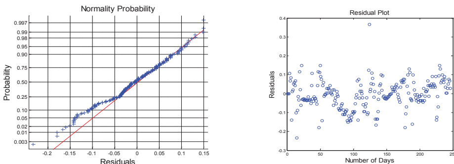
Fig. 4: Normal Probability Plot and Residual Plot
