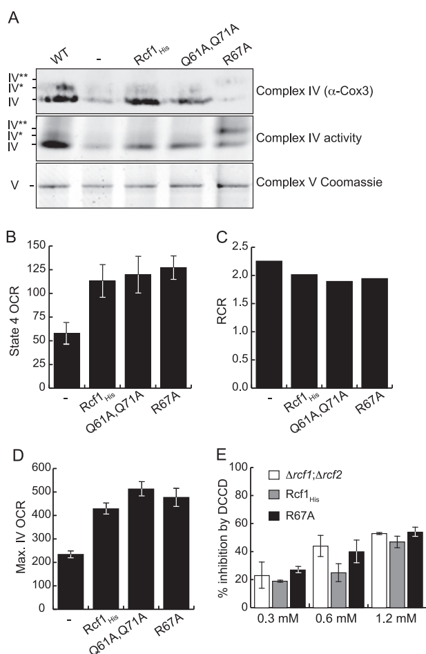
FIGURE 5. Complex IV in rcf1_{His}^{R67A} mitochondria displays altered catalytic properties. A, mitochondria isolated from WT or the \Delta rcf1;\Delta rcf2 strain harboring the Rcf1 His , rcf1_{His}^{Q61A,Q71A} , rcf1_{His}^{R67A} derivatives, as indicated, were solubilized with DDM (0.6%) and subjected to duplicate BN-PAGE analysis. The complex IV enzyme activity levels were analyzed in one set of samples by performing an in-gel enzyme activity assay (center panel), and in a parallel sample, the complex IV protein levels were determining following Western blotting and decoration with Cox3 antibody (top panel), as indicated. The levels of Coomassie-stained complex V ( F_1F_0 -ATP synthase) are shown in the bottom panel as a loading control. B and C, the OCRs of the NADH-driven state 4 and respiratory control ratio (the ratio of state 3 (NADH/ADP) to state 4 (NADH)) were measured in the indicated isolated mitochondria ( n = 3 ). D, the maximal capacity of complex IV was determined by measuring the OCR driven by ascorbate/TMPD in the presence of CCCP to dissipate the membrane potential ( n = 6 ). E, isolated \Delta rcf1;\Delta rcf2 mitochondria and \Delta rcf1;\Delta rcf2 harboring the Rcf1 His or rcf1_{His}^{R67A} derivatives were incubated with DCCD at the indicated concentrations for 90 min at room temperature prior to measuring the maximal complex IV OCR in the presence of ascorbate/TMPD and CCCP. The percent of inhibition caused by the DCCD treatment relative to the control (no DCCD) is indicated.
