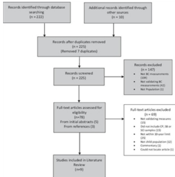
Figure 1. PRISMA Diagram.
