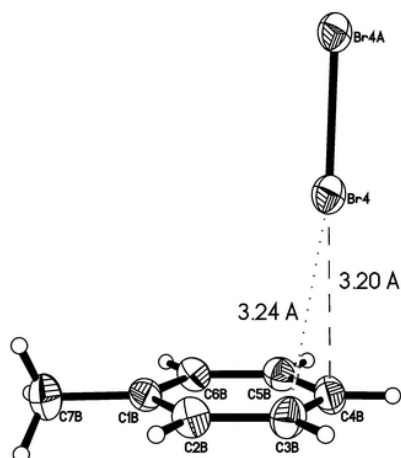
Fig. 4 Localized bonding of bromine to the ortho - (top) and para - (bottom) centers of toluene in the charge-transfer complex.
