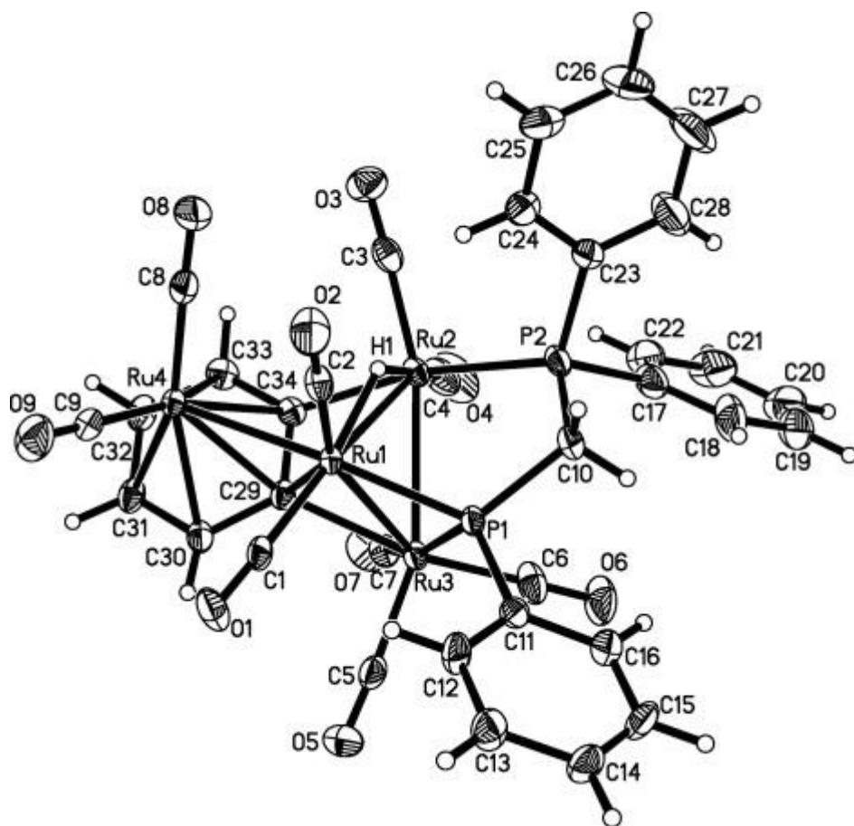
Fig. 3. The solid-state molecular structure of [\text{Ru}_4(\text{CO})_9(\mu_3\text{-}\eta^2\text{-PhPCH}_2\text{PPh}_2)(\mu_4\text{-}\eta^6:\eta^1:\eta^1:\eta^1\text{-C}_6\text{H}_4)(\mu\text{-H})] ( 7 ).
