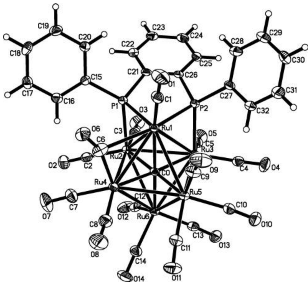
Fig. 1. The solid-state molecular structure of [\text{Ru}_6(\mu\text{-CO})(\text{CO})_{13}\{\mu_4\text{-PhP}(\text{C}_6\text{H}_4)\text{PPh}\}(\mu_6\text{-C})] ( 5 ).
