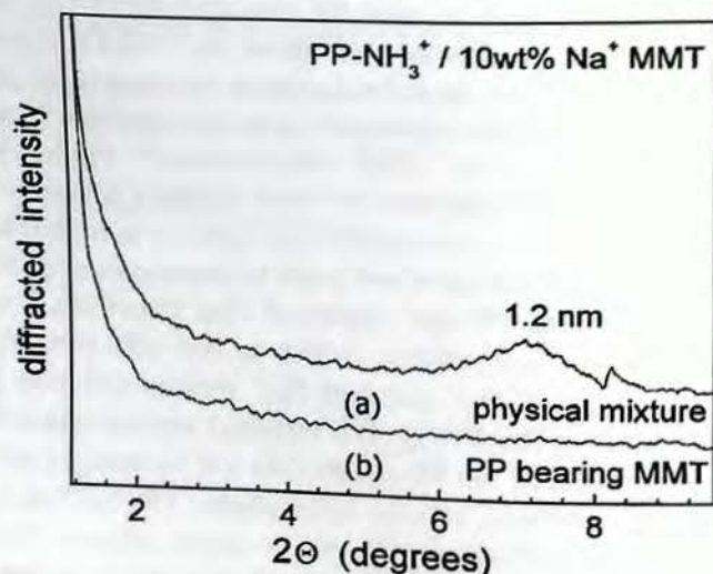
Fig. 15. X-ray diffraction patterns of PP- t - NH_3^+Cl^-/Na^+ -MMT (90/10 weight ratio): (a) physical mixture by simple powder mixing at ambient temperature and (b) the same mixture after static melt-intercalation. Reprinted with permission from [33], Z. M. Wang et al., Macromolecules 36, 8919 (2003). © 2003, American Chemical Society.
