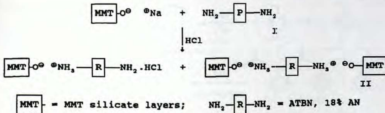
Fig. 3. Preparation of the rubber-MMT material. Reprinted with permission from [46], A. Akelah et al, Mater. Lett. 22, 97 (1995). © 1995, Elsevier.
