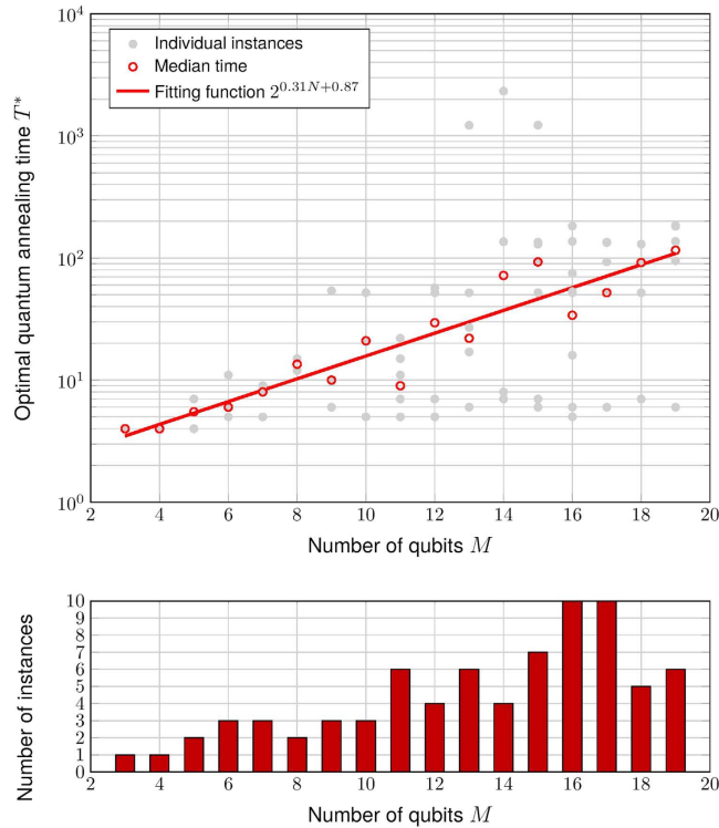
Figure 3. Plot of the optimal quantum annealing time T^* versus the number of spins involved in the construction of H_{SCP} . Here we fit the logarithm of median T^* with a straight line. The size M of our Ising systems ranges from 3 to 19. From the fitting function we observe that the annealing time scales as roughly O(2^{0.31M}) . We also provide on the bottom plot the number of instances for each M .
