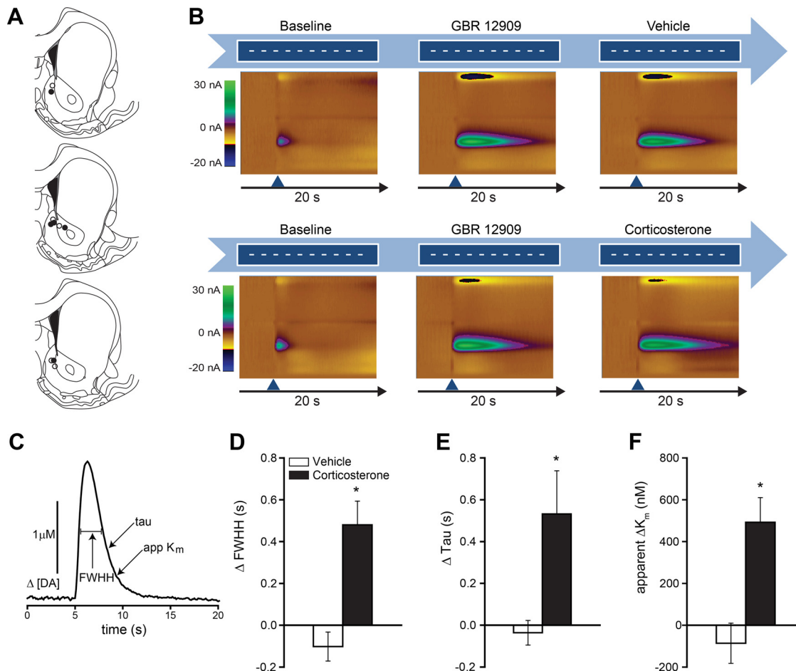
Figure 4. Corticosterone administration decreases dopamine uptake after DAT blockade. A , NAC recording sites for dopamine uptake measurements in vehicle-treated ( \circ ) and corticosterone-treated ( \bullet ) rats. B , Experimental design and example of two-dimensional color representation of cyclic voltammetric data collected for 20 s around a single stimulation. The ordinate is the applied voltage ( E_{app} ), and the abscissa is time (in seconds). Changes in current at the carbon-fiber electrode are indicated in color. After 10 baseline stimulations (white horizontal lines), rats were injected with GBR12909 (15 mg/kg) and stimulated until stabilization of the drug response (center color plot). Rats were then either injected with corticosterone (2 mg/kg, n = 5 , right color plot, top), or vehicle ( n = 5 , right color plot, bottom). C , Measures of dopamine uptake. D–F , Mean \pm SEM change in measures of uptake after corticosterone treatment ( D , FWHH; E , \tau ; and F , apparent K_m ), compared with vehicle-injected controls. * p < 0.05 , compared with vehicle (Student's unpaired t test).
