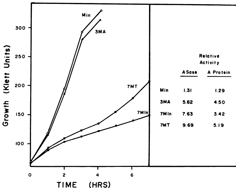
FIG. 4. Derepression and growth inhibition by 3-methylanthranilic acid (3MA), 7-methylindole (7Min), and 7-methyltryptophan (7MT) in W1485 tna . Cultures were harvested at the end of the growth period and cell-free extracts were prepared. Enzyme activities are relative to the level of enzymes in W1485 tna grown in minimal medium.
