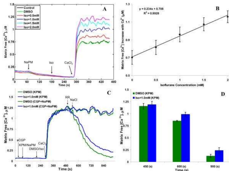
Figure 7 (A) Time-course of mitochondrial free Ca^{2+} ( [Ca^{2+}]_m ) with 0.5 mM added CaCl_2 ( \approx 200 nM free Ca^{2+} ) during state 2 respiration with Na^+ -pyruvate/malate (NaPM) and isoflurane (0.5, 1, 1.5 and 2 mM) compared to control (no treatment) and
