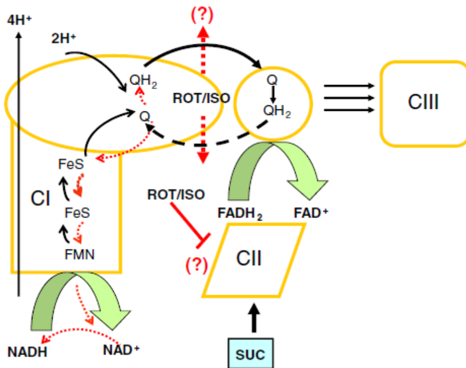
Fig. 8. Schema depicting electron transfer from substrate SUC to downstream and upstream complex I and complex III, respectively. Electrons from SUC pass through FADH 2 to the Q pool, which transfers electrons to the Q site of complex I. Within complex I, electrons transferred to the Q site can either go in the reverse direction via RET through FeS clusters and FMN to generate NADH from NAD + or go in the forward direction via FET to produce QH 2 ; RET vs. FET is dependent on the standard reduction potential across complex I. Binding of ISO, like ROT, may inhibit the transfer of electrons from the QH 2 of complex I to the Q pool to complex III. Solid arrows (→) show electrons transported in the forward direction (FET) and broken arrows (⇌) show electrons transported in the reverse direction (RET). Question marks (?) show the possible indirect mechanisms of attenuation in FET either via attenuation of electron transfer from the Q site of complex I to the Q pool, or succinate generated accumulation of oxaloacetate due to ROT/ISO mediated decrease in NADH oxidation.
