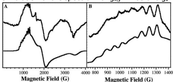
Figure 5 (A) Top: EPR spectrum of [Co_(E151A-AAP)] in HEPES buffer, pH 7.50 recorded at 10 K, 0.2 mW microwave power, 12.6 G field modulation amplitude, 100 kHz modulation frequency. Bottom: simulation of the EPR spectrum of [Co_(E151A-AAP)] with three species: (1) g_{x,y} = 2.509 , g_z \approx 2.19 , E/D = 0.19 , A = 0.0069 \text{ cm}^{-1} ; (2) g_{x,y} = 2.565 , g_z \approx 2.19 , E/D = 0.20 , A = 0.0082 \text{ cm}^{-1} ; (3) g_{x,y} = 2.29 , g_z \approx 2.55 , E/D = 0.08 . (B) Low-field region of the spectrum recorded at higher resolution and a correspondingly expanded view of the simulation.
