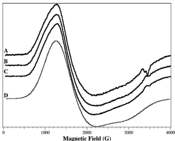
Figure 4 EPR spectra of metal-reconstituted E151D-AAP, pH 7.50. All spectra were recorded at 10 K, 0.2 mW microwave power, 12.6 G field modulation amplitude, 100 kHz modulation frequency. (A) EPR spectrum of [CoZn(E151D-AAP)]; (B) EPR spectrum of [ZnCo(E151D-AAP)]; (C) EPR spectrum of [CoCo(E151D-AAP)]; (D) simulation of the spectra with g_{x,y} = 2.35 and g_z = 2.38 , E/D = 0.1 .
