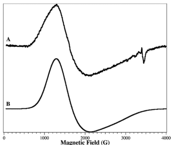
Figure 6 Top: EPR spectrum of [(\text{CoCo}(\text{E151A-AAP}))] in HEPES buffer, pH 7.50 recorded at 10 K, 0.2 mW microwave power, 12.6 G field modulation amplitude, 100 kHz modulation frequency. Bottom: simulation of the EPR spectrum of [\text{CoCo}(\text{E151A-AAP})] with g_{x,y} = 2.29 , g_z \approx 2.55 , E/D = 0.08 .
