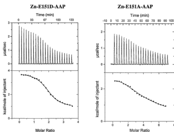
Figure 2 Isothermal titration data for the titration of (A) apo-E151D-AAP and (B) apo-E151A-AAP with Zn(II) (50 mM HEPES buffer pH 7.5 at 25 °C).
