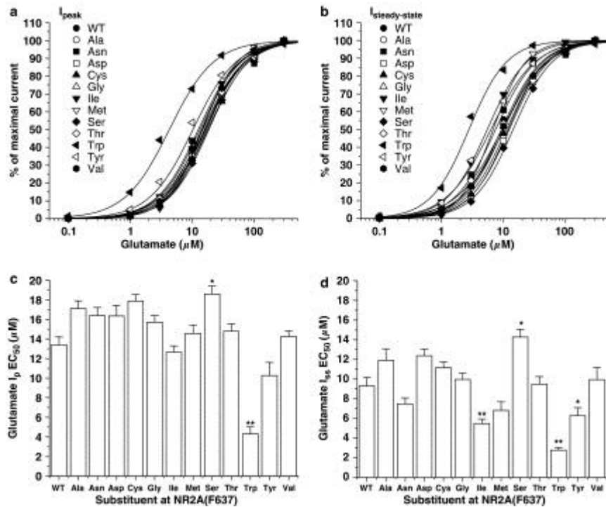
Figure 3. NR2A(F637) mutations can alter EC_{50} values for both peak and steady-state glutamate-activated current. Concentration–response curves for glutamate (in the presence of 50 \mu\text{M} glycine) activation of peak (a) and steady-state (b) current in lifted human embryonic kidney 293 cells expressing NR1/NR2A or NR1/NR2A(F637) mutant subunits. Data points are means of five to eight cells and curves shown are the least-squares fits to the equation given in Materials and methods. Bar graphs show peak (c) and steady-state (d) EC_{50} values for glutamate in lifted cells expressing the various NR2A(F637) mutant subunits. Asterisks indicate EC_{50} values that differed significantly (ANOVA and Dunnett's test; * P < 0.05 , ** P < 0.01 ) from the EC_{50} for wild-type NR1/NR2A subunits.
