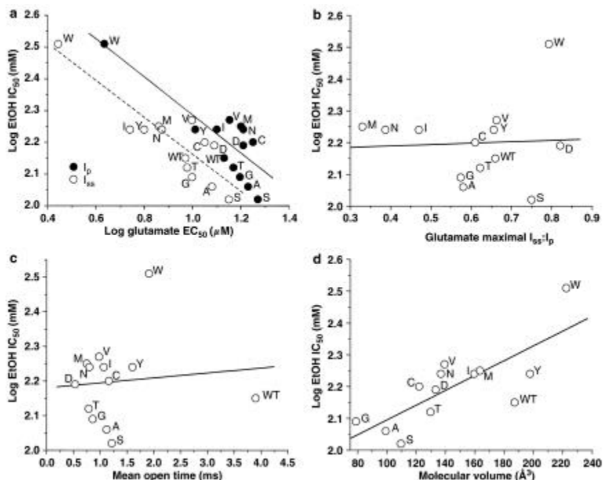
Figure 7. Relation of agonist potency, ion channel gating and substituent molecular volume to EtOH sensitivity in NMDA receptors containing NR2A(F637) mutant subunits. Graphs plot log IC_{50} for EtOH vs log EC_{50} values for glutamate peak and steady-state current ( a ) maximal I_{ss}:I_p for glutamate ( b ), mean open time ( c ) and substituent molecular volume in \text{\AA}^3 ( d ) for the various substituents at NR2A(F637). Data points are labeled with the substituted amino acid for the various mutants at NR2A(F637). The lines shown are the least squares fits to the data. Highly significant correlations were obtained between log EtOH IC_{50} and log EC_{50} for glutamate activation of peak ( R^2=0.626 , P<0.001 ) and steady-state ( R^2=0.743 , P<0.0001 ) current, but not glutamate maximal I_{ss}:I_p ( R^2=0.001 , P>0.05 ) or mean open time ( R^2=0.006 , P>0.05 ). A significant linear relation was obtained between log EtOH IC_{50} and molecular volume ( R^2=0.587 ; P<0.005 ), but not hydrophathy ( R^2=0.001 , P>0.05 ), polarity ( R^2=0.003 , P>0.05 ) or hydrophilicity ( R^2=0.276 , P>0.05 ).
