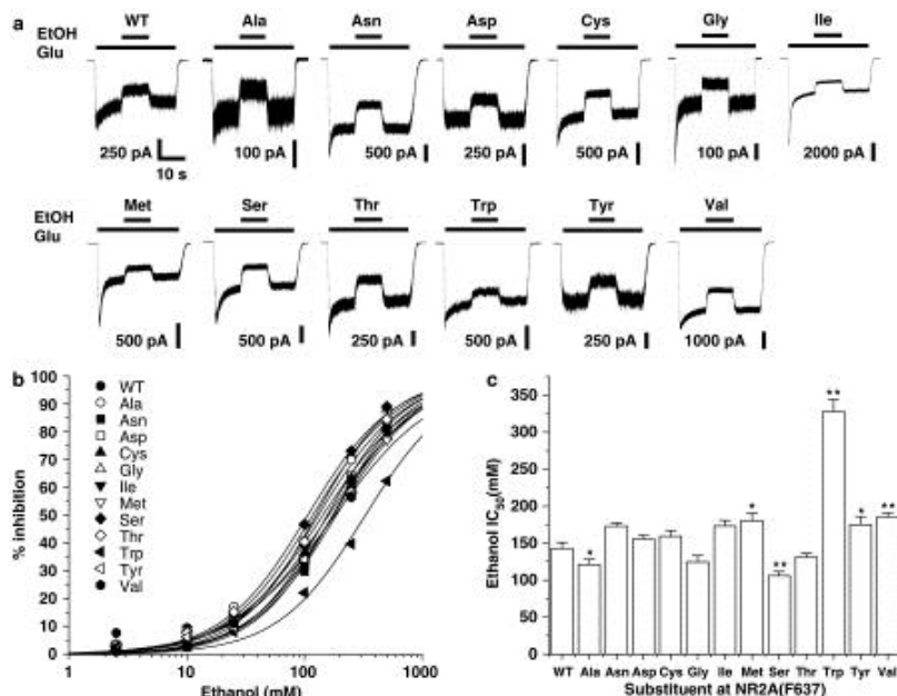
Figure 2. Effect of EtOH on NMDA-activated current in cells expressing NR2A(F637) mutant subunits. (a) Records are currents activated by 10 μM glutamate (Glu) and 50 μM glycine in the absence and presence of 100 mM EtOH in human embryonic kidney (HEK) 293 cells coexpressing NR1 and wild-type (WT) NR2A or various NR2A(F637) substitution mutant subunits. (b) Concentration–response curves for EtOH inhibition of current activated by 10 μM glutamate (Glu) and 50 μM glycine in HEK 293 cells coexpressing NR1 and wild-type NR2A (WT) or various NR2A(F637) substitution mutant subunits. Data points are means of five to 12 cells and curves shown are the least-squares fits to the equation given in Materials and methods. (c) Bar graph shows IC 50 values for EtOH in cells expressing the various NR2A(F637) mutant subunits. Asterisks indicate IC 50 values that differed significantly (ANOVA and Dunnett's test; *P<0.05, **P<0.01) from the IC 50 for WT NR1/NR2A subunits.
