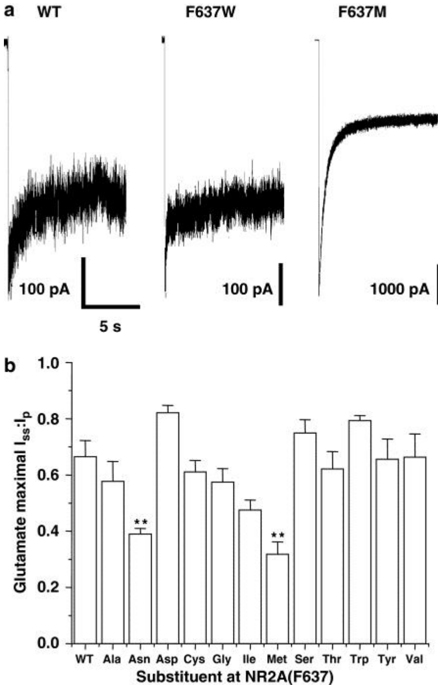
Figure 4. Effect of NR2A(F637) mutations on desensitization kinetics. (a) Traces illustrating desensitization of current activated by 300 \mu\text{M} glutamate (in the presence of 50 \mu\text{M} glycine) in lifted cells expressing wild-type (WT) NR1/NR2A, NR1/NR2A(F637W) and NR1/NR2A(F637M) subunits. (b) Average values of I_{ss}:I_p of glutamate-activated current; n=5-8 cells. Asterisks indicate values that differed significantly (ANOVA and Dunnett's test; **P<0.01 ) from the value for WT NR1/NR2A subunits.
