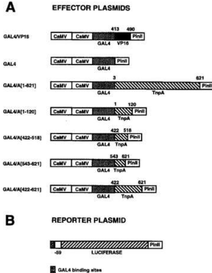
Figure 1: Schematic representation of the GAL4 fusion genes and the luciferase reporter gene.
