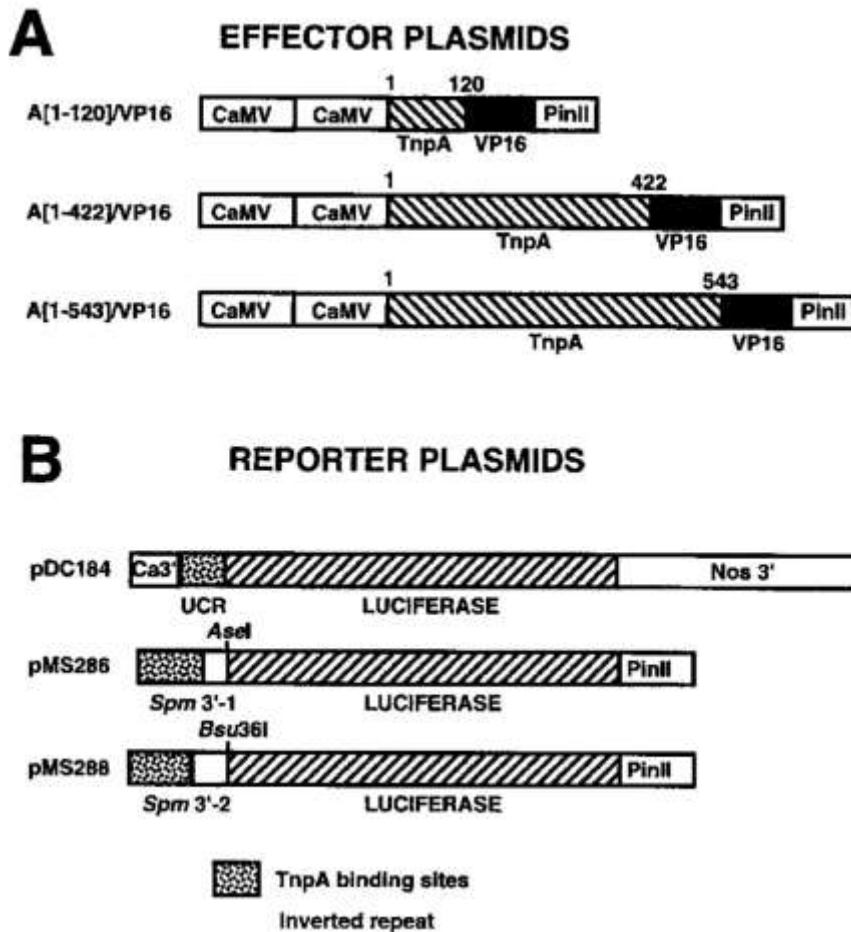
Figure 3: Schematic representation of chimeric TnpA-VP16 and Spm promoter-luciferase reporter genes.
