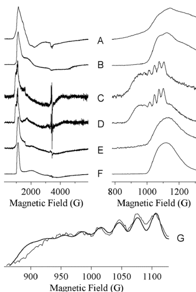
Figure 2 EPR spectra of 1 mM Co–VanX in the resting state (A, B), after 10 ms reaction with 5 mM d-ala-d-ala (C, D), and after complete reaction with d-ala-d-ala (E, F). The traces in G show the hyperfine region of spectrum C with a simulation overlaid indicating A^I = 7/2(^{59}\text{Co}) = 3.5 \times 10^{-3} \text{ cm}^{-1} (33 G). Spectra A, C, E, and G were recorded at 9.63 GHz, 11 K, 2 mW; B, D, and F were recorded at 5 K, 200 mW.
