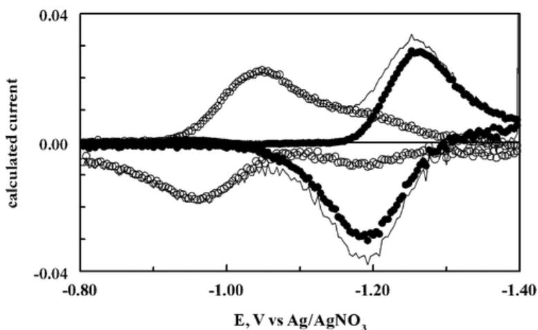
Figure 3. DCVA calculated from the concentrations of DNB, DNB •- , and DNB 2- from Figure S3. The open circles are due to the first reduction, closed circles are due to the second reduction alone, and the solid line is the total calculated DCVA current. Scan rate = 2.0 mV/s. Solvent: acetonitrile. Electrolyte: 0.10 M TBAP.
