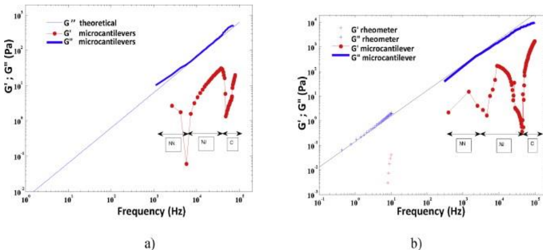
Figure 9. a) Rheogram of water (1cP) measured with three microcantilevers (LL, LH and A) and using Eqs. 16-18, b) Rheogram of silicone oil (20cP) measured with
