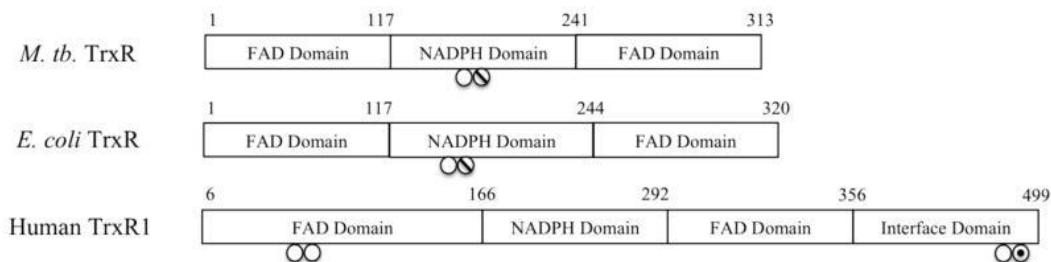
Figure 6 Comparison of the three thioredoxin reductases discussed in this study. The M. tuberculosis . TrxR shows 45% identity and 63% homology to the E. coli TrxR
