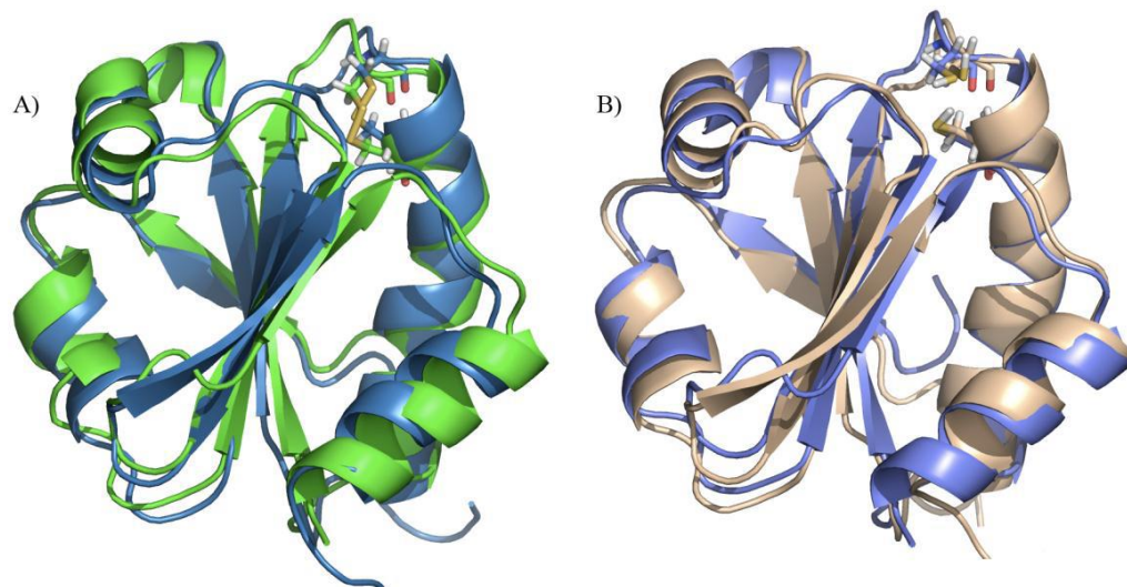
Figure S1. Overlays of both redox states of solution structures from E. coli Trx and M. tuberculosis TrxC, where A) is the overlay for the oxidized states, with blue being from M. tuberculosis and green from E. coli and B) is the overlay for the reduced states, with wheat being from M. tb and purple from E. coli .
