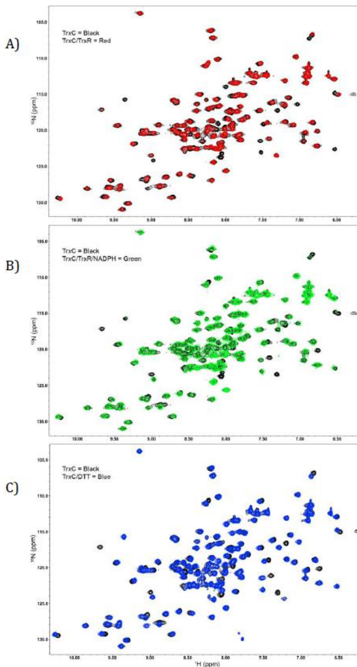
Figure S2. 2D ^1\text{H} - ^{15}\text{N} HSQC spectra where the black cross peaks in all panels are for oxidized/reduced TrxC and A) TrxR has been added to the sample (red), B) TrxR has been added to the sample and the redox activity initiated by addition of with NADPH to reduce TrxC (green), and C) DTT is added to the sample to fully reduce TrxC as a control experiment (blue). Protein concentration is 250\ \mu\text{M} for TrxC and TrxR is slightly less than 250\ \mu\text{M} .
