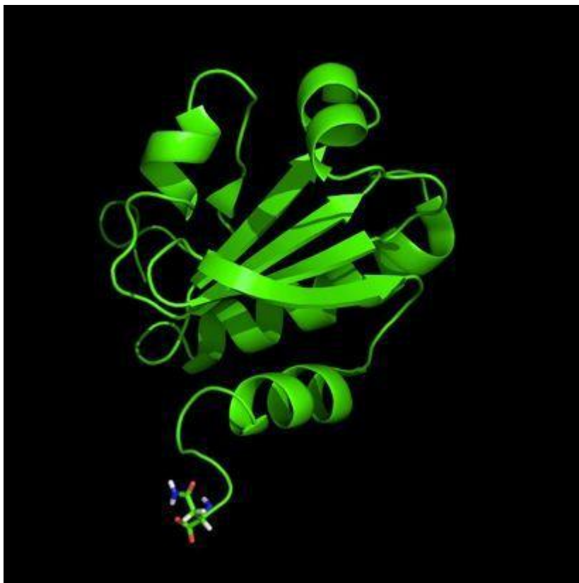
Figure S4. Structure of TrxC showing location of last contiguously assigned residue, Asn116. The C-terminal histidine tag was present after Asn116 (some residues in the histidine tag were assigned as well).
