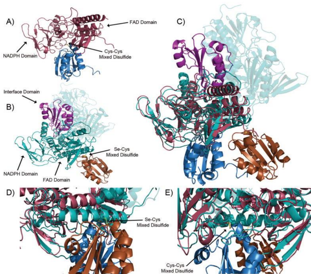
Figure 5 Comparison of the M. tuberculosis . and human Trx-TrxR complex. (a) M. tuberculosis . Trx (blue)-TrxR (red) mixed disulfide. (b) Human Trx (orange)-TrxR (teal) mixed disulfide. Note the carboxy-terminus of the dimer pair is highlighted in violet and forms the mixed disulfide. (c) Overlay of the M. tuberculosis . and human thioredoxin systems. (d) Close up of M. tuberculosis thioredoxin complex disulfide from Figure 5(c). (e) Close up of the human thioredoxin complex disulfide from Figure 5(c).
