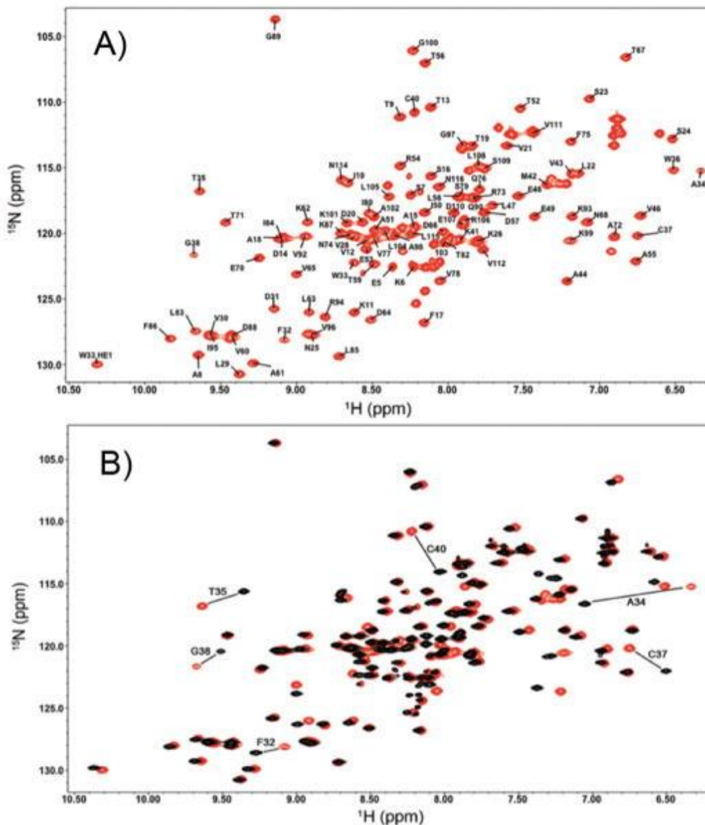
Figure 2 2D ^1\text{H} - ^{15}\text{N} HSQC spectra of (a) the oxidized state of TrxC (red) with all the backbone N-H chemical shifts assigned, and (b) the oxidized (red) and reduced (black) states of TrxC, with the large chemical shift changes associated with disulfide reduction labeled.
