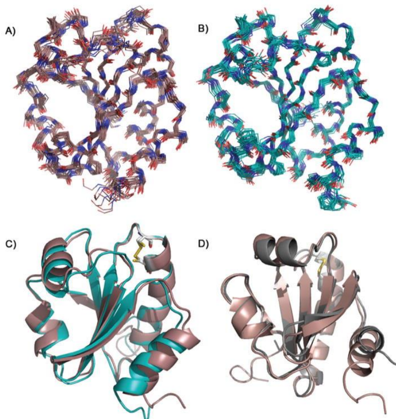
Figure 1 Solution NMR structures of TrxC: (a) the ensemble for oxidized TrxC with a backbone RMSD of 0.54 Å, (b) the ensemble for the reduced state of TrxC with a backbone RMSD of 0.50 Å, and (c) overlay of the median structures for both redox states, colored as in panels (a) and (b). Note: disordered N- and C-terminal residues 1–6 and 113–116 have been omitted for clarity in panels (a) and (b). (d) Overlay of the median NMR solution structure for the oxidized TrxC (red) and the crystal structure of oxidized TrxC (gray), with the active site disulfides shown in yellow. The only significant deviation is in the C-terminal helix, \alpha_4 , which in the crystal structure participated in an interaction with another TrxC in the asymmetric unit.
