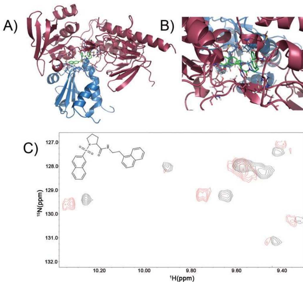
Figure 7 (a) Result of docking into one of the intermediates in the thioredoxin catalytic cycle, to demonstrate the presence of potential binding pockets at the Trx/TrxR interface of sufficient size to accommodate potential inhibitors or drug leads. After docking 10,000 compounds, the best scoring (lowest energy) docked structure (shown in green, compound number CSDDD_6702) occupied a site at the interface of TrxR (red) and TrxC (blue) in Panels A and B, with energy = -10 kcal/mol using AutoDock4. (b) Expansion that shows the docking pose for CSDDD_6702. (c) Expansion showing the crosspeak perturbations in a section of the 15 N- 1 H HSQC upon addition of 200 \mu M of compound CSDDD_6702 (blue) to a sample containing 200 \mu M TrxC, 250 \mu M TrxR, and 0.80 mM NADPH (black). Interface residue W33(HE1) is represented by the crosspeak at 10.2 ppm, which has been shifted upon binding CSDDD-6702.
