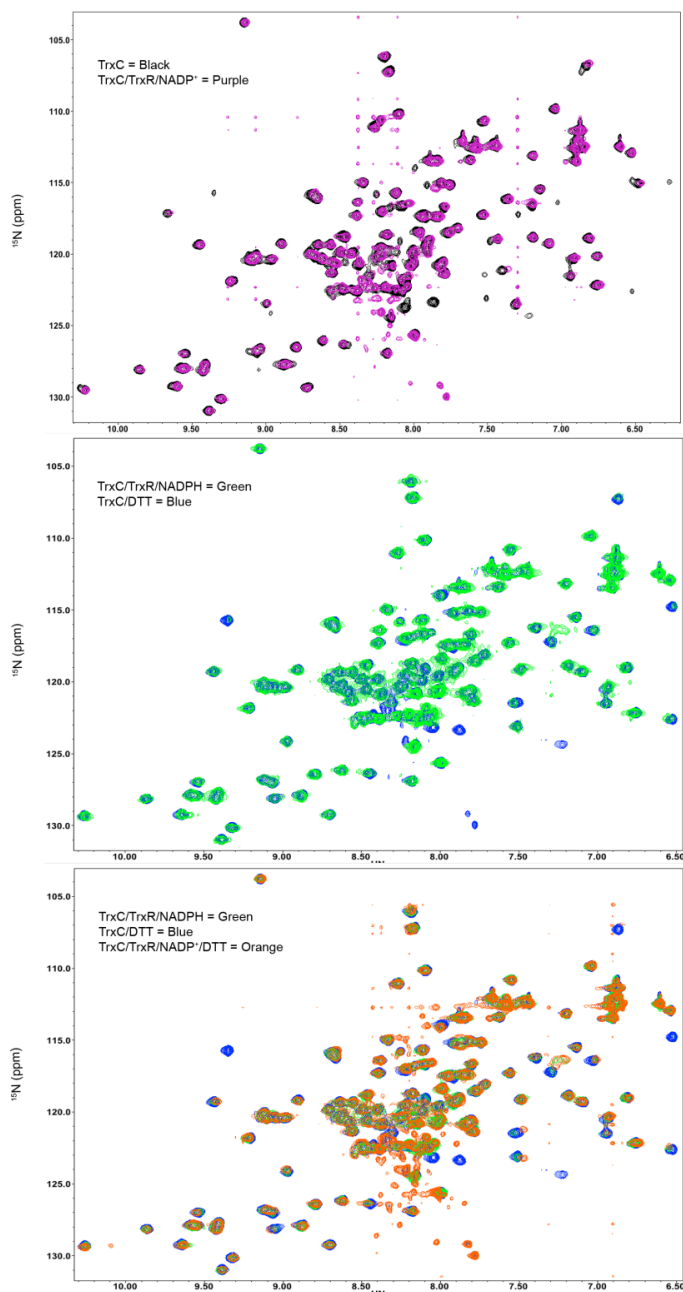
Figure S2 continued. 2D ^1\text{H} - ^{15}\text{N} HSQC spectra where D) black cross peaks are for oxidized/reduced TrxC and TrxR is added to the sample along with the oxidized cofactor NADP + . E) The overlay of the DTT reduced sample (blue) and the NADPH reduced sample (green), and F) is the same as panel E with the oxidized sample from panel D and DTT added to it (orange).
