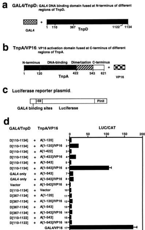
Figure 5 Analysis of TnpA–TnpD interactions in a plant two-hybrid system. (a–b) Schematic representations of the components from which the fusion constructs were assembled. Each contained either the GAL4 DNA binding domain or the VP16 transcription activation domain but different segments of
