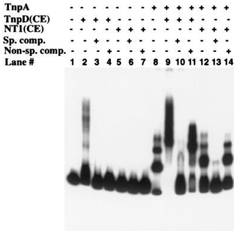
Figure 4 Binding of TnpD to DNA and DNA–TnpA complexes. A 279-bp DNA fragment containing two TnpA binding sites was used as the binding target DNA (Fig. (Fig.11b)). Binding reactions were performed in DNA binding buffer and contained 80 ng of TnpA and 10 µg of protein from cell extracts. The
