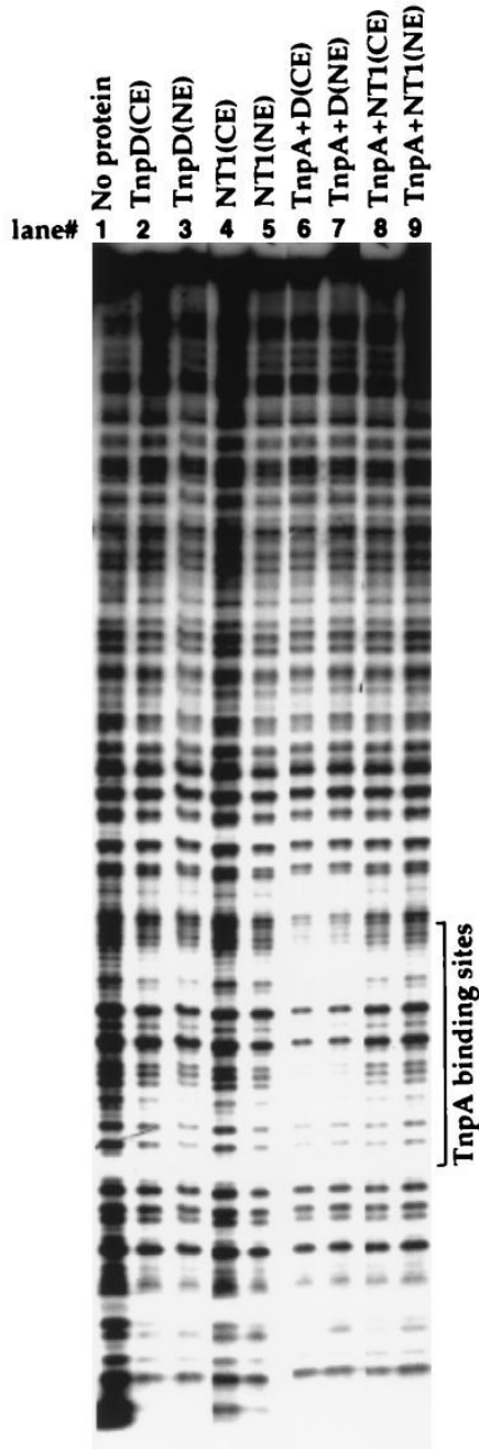
Figure 6 DNase I footprint analysis of protein–DNA complexes. A labeled DNA fragment containing a tail-to-tail dimeric TnpA binding motif was incubated with the proteins indicated at the top of each lane before digestion with DNase I. The digested products were fractionated on a denaturing 8% polyacrylamide gel. TnpD (CE) and TnpD(NE) were whole cell and nuclear extracts, respectively, of transgenic tobacco cells expressing TnpD from CaMV 35S promoter; NT1(CE) and NT1(NE) were whole cell and nuclear extracts,
