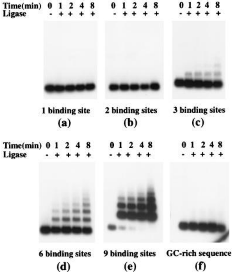
Figure 2 TnpA-mediated formation of DNA multimers in the presence of ligase. ^{32}\text{P} -labeled DNA fragments (20 ng) containing (a–e) or lacking (f, the GC-rich region of Spm ) TnpA binding sites were incubated with 120 ng of TnpA in the presence or absence of ligase for the time indicated, were deproteinized, were fractionated on a 1% agarose gel, and were detected by autoradiography.
