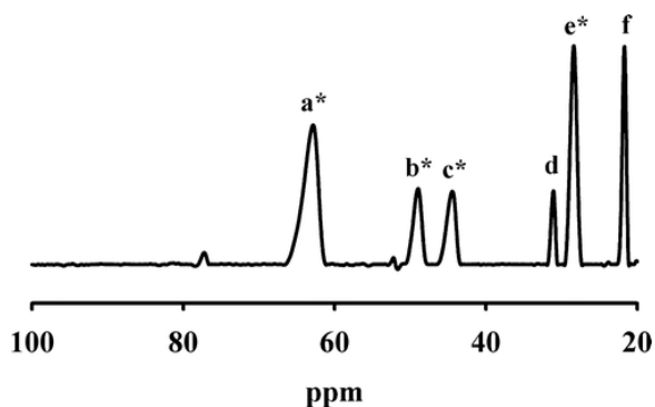
Figure 4. 1 H NMR spectrum of the 2Co-R246H mutant of GLX2-1 in 10 mM MOPS, pH 7.2, containing 10% D 2 O. The enzyme concentration in the samples was ~1 mM. The * represents peaks that were solvent-exchangeable. Peak e in the spectrum decreased by one-half when the sample was exchanged in 90% D 2 O.
