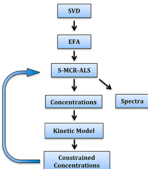
Figure 1. HS-MCR-ALS approach.
