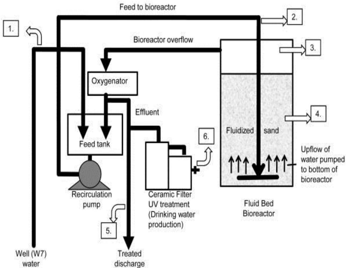
Figure 1 Schematic diagram of Bioreactor #1. The fluidized-bed medium in this reactor was sand. Sampling points are indicated with arrows: 1. influent; 2. bioreactor influent; 3. effluent; 4. sand; 5. treated discharge; 6. UV-treated effluent.
