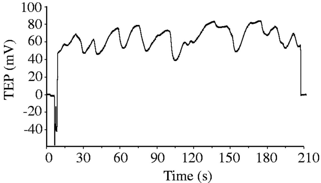
Fig. 1. Representative recording from a Malpighian tubule showing transepithelial potential (TEP) oscillations. At the beginning of the trace, the electrode is in the bath. The negative deflection reflects the potential across the basolateral membrane of a principal cell as the electrode enters the cell; as the electrode is advanced into the lumen of the tubule, the recorded potential becomes positive. At the end of the trace, the electrode is withdrawn into the bath again.
