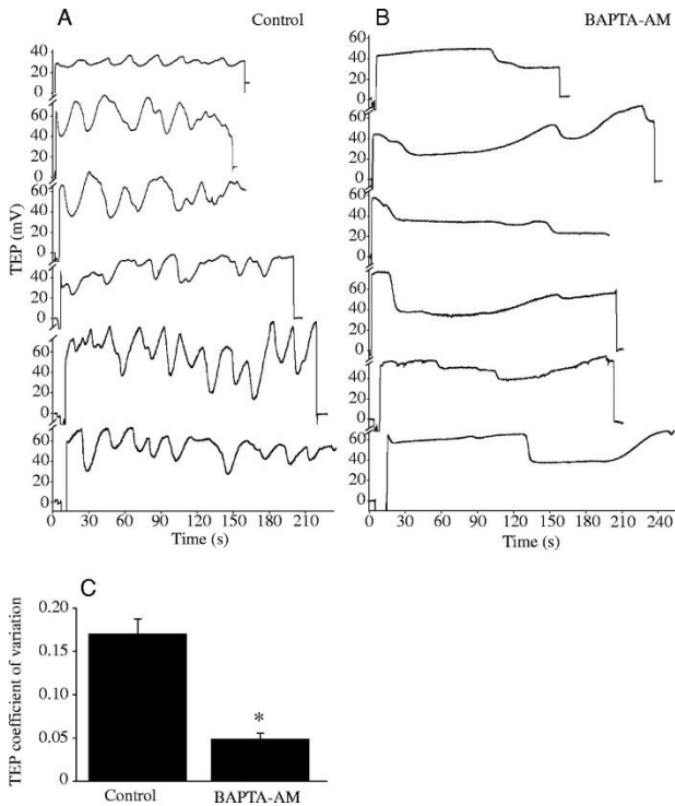
Fig. 5. Dependence of TEP oscillations on intracellular calcium. Traces from six control (A) and six BAPTA-AM loaded (B) tubules are shown. (C) Quantification of the effect of BAPTA on the coefficient of variation for the 12 traces shown in A and B. See text for details of methods. Values are means \pm s.e.m., * P < 0.0001 (paired t -test).
