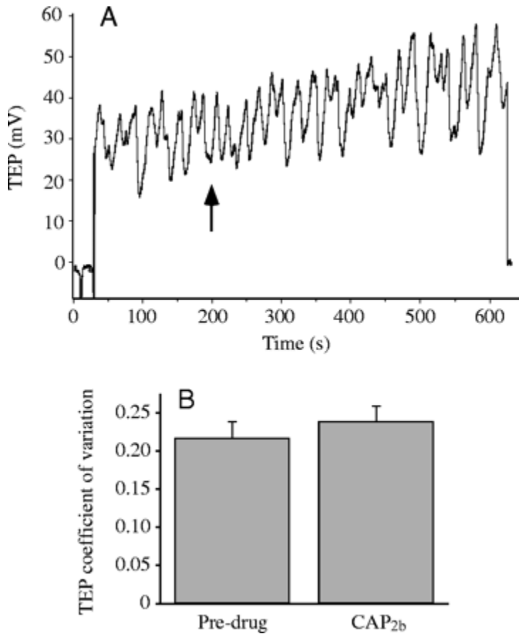
Fig. 9. CAP 2b does not alter the oscillations. (A) Trace from a tubule exposed to 100nmol -1 CAP 2b starting at the arrow. Note the lack of any immediate effect of the drug on the TEP. Similar results were seen in five additional tubules. (B) Graph showing no effect of CAP 2b on TEP variability. The TEP coefficient of variation was measured before drug application and during exposure to 100nmol -1 CAP 2b lasting 5.5–11min. Values are means \pm s.e.m., N=6 tubules, P>0.14 (paired t -test).
