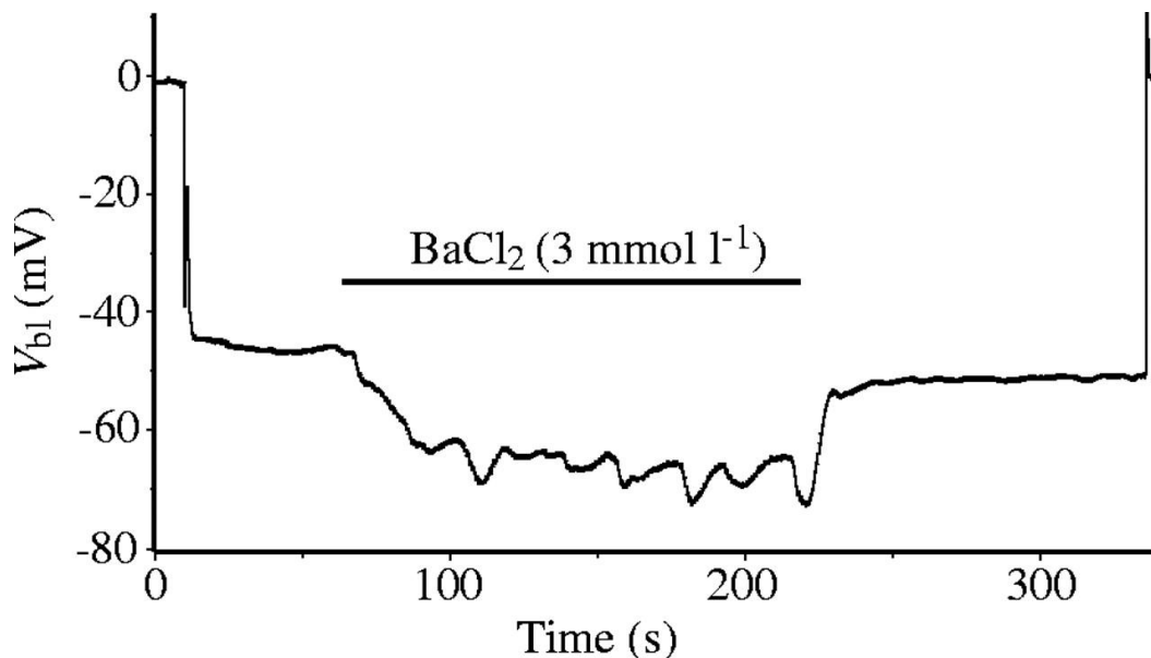
Fig. 2. Effect of \text{Ba}^{2+} on principal cell basolateral membrane potential. The electrode is positioned inside a principal cell. Application of 3\text{mmol l}^{-1} \text{BaCl}_2 for the duration indicated by the bar results in a hyperpolarization of V_{bl} and the appearance of voltage oscillations. Similar results were seen in two additional tubules.
