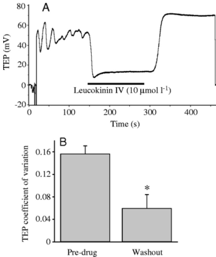
Fig. 8. Effect of leucokinin on TEP oscillations. (A) Addition of leucokinin IV ( 10\mu\text{mol l}^{-1} ) rapidly depolarizes the TEP. After drug washout, the TEP recovers amplitude while the oscillations remain inhibited. (B) Average results from six tubules show long-lasting inhibition of oscillations after leucokinin washout. Values are means \pm s.e.m., *P<0.01 (paired t -test). Inhibition of oscillations was measured beginning 60s after washout following an application of 10\mu\text{mol l}^{-1} leucokinin lasting 25–140s.
