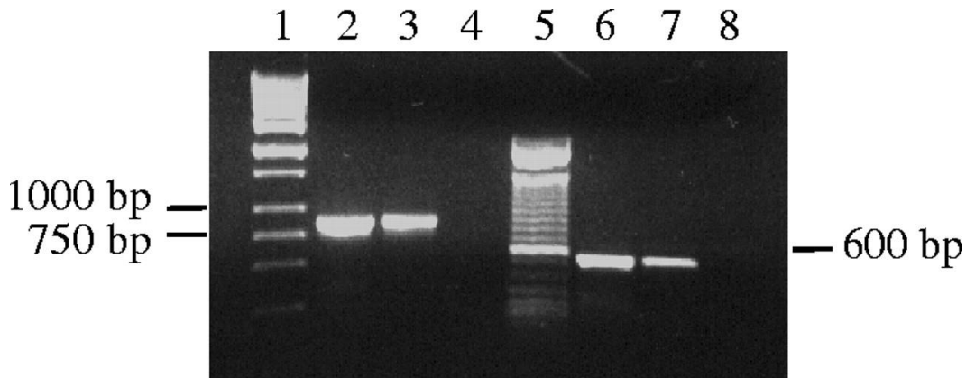
Fig. 7. Expression of genes encoding intracellular calcium-release channels in the tubule. The gel shows the result of RT-PCR from whole-fly mRNA (lanes 2,6) and tubule-specific mRNA (lanes 3,4,7,8) using primers specific to the IP 3 receptor (IP 3 R) (lanes 2–4) and the ryanodine receptor (RyR) (lanes 6–8). In lanes 4 and 8, reverse transcriptase was omitted from the cDNA synthesis reaction to control for possible genomic DNA contamination. The PCR reactions give products of the expected sizes: 547base pairs (bp) for RyR, compared to 678bp from genomic DNA, due to the inclusion of two short introns (Adams et al., 2000) and 843bp for IP 3 R (Sinha and Hasan, 1999). Because the 5' IP 3 R primer spans an exon–intron junction, genomic DNA should not give any PCR product. Lane 1: 1kb ladder (Stratagene, La Jolla, CA, USA); Lane 5: 100bp ladder (Life Technologies).
