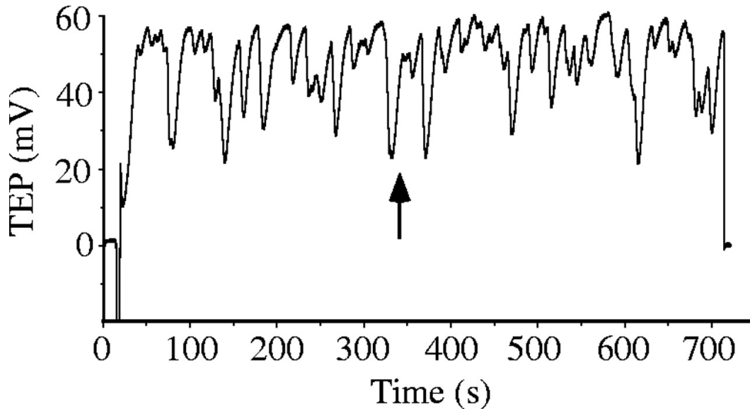
Fig. 6. Lack of dependence of TEP oscillations on peritubular calcium. In the trace shown, the tubule is bathed in a normal, calcium-containing saline. At the arrow, the bathing solution is switched to a nominally calcium-free saline. Similar results were obtained from seven other tubules.
