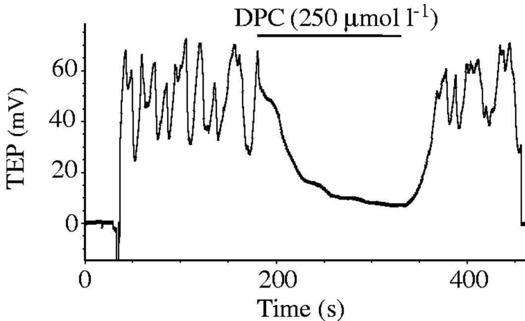
Fig. 4. Effect of DPC on tubule electrophysiology. Application of 250\mu\text{mol l}^{-1} DPC (bar) rapidly depolarizes the TEP, which recovers upon washout of the drug. Similar results were seen in four additional tubules (see Table1).
