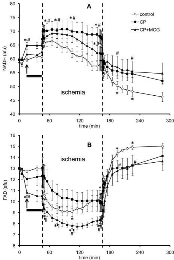
Figure 2 Time course of changes in NADH autofluorescence (A) and FAD autofluorescence (B) at baseline, during treatment, hypothermia, cold ischemia, and warm reperfusion in control (n=5), CP (n=5), and CP+MCG (n=5) groups. The arrow indicates where the data point was recorded during treatment at 37°C. The solid horizontal bar indicates the period of treatment at 27°C. The period between the two unbroken vertical lines refers to ischemia. * P < 0.05 values vs. baseline within each group; # P < 0.05 each treatment vs. the control group; ¶ P < 0.05 , CP+MCG vs. CP alone.
