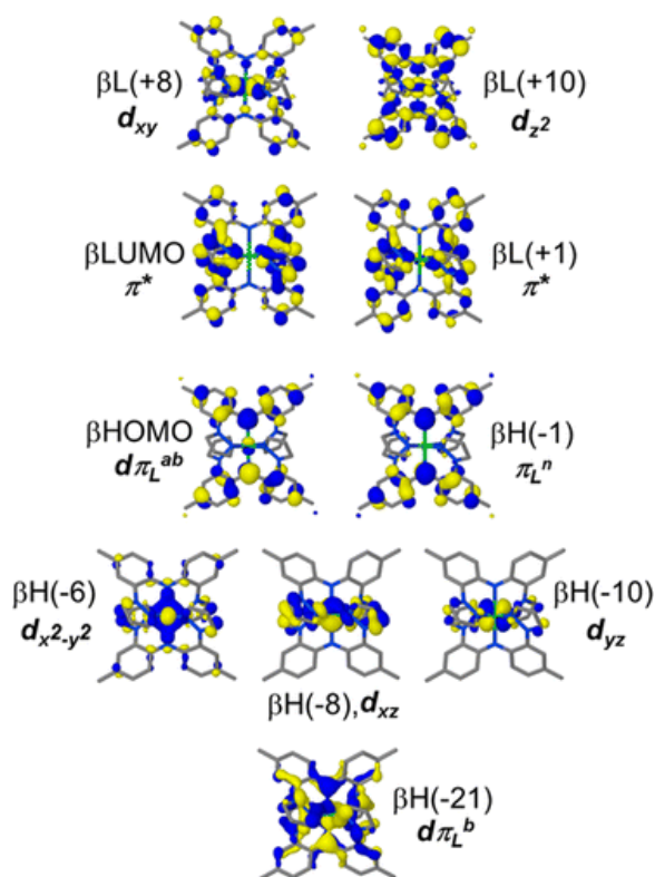
Figure 3. \beta -Frontier orbitals of \text{Ni}(\text{Me},\text{Me})_2 calculated at the M06/def2-SV(P) level.
