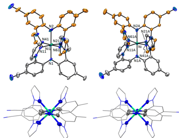
Figure 2. Top: Structures of the two isomers ( cis -isomer, left; trans -isomer, right) of Ni(Me,CN) 2 found in the crystal with partial atom labeling. Hydrogen atoms have been removed, and carbon atoms of the top ligand on each complex have been colored gold for clarity. Bottom: Views approximately down N1–Ni–N2 bonds showing the nearly planar amido “(N Ar ) 2 NiC 4 ” moiety.
