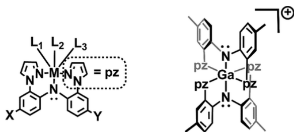
Figure 1. Metal complexes of pyrazolyl-containing redox-active pincer ligands.
