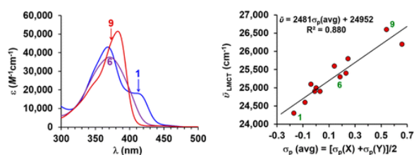
Figure 4. Left: Overlay of higher energy portion of the UV–vis spectrum of 1 (blue), 6 (violet), and 9 (red). Right: Plot showing correlation between energy ( cm^{-1} ) of LMCT transition and the average of the Hammett \sigma_p parameter of X and Y para -aryl substituents in Ni(X,Y) 2 complexes 1–12 .
