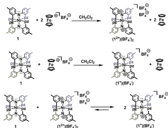
Scheme 2. Preparation of Oxidized [Ni(Me,Me) 2 ] n+ ( n = 1, 2) Complexes
