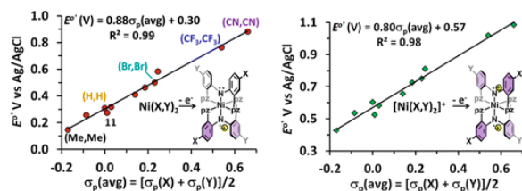
Figure 7. Correlations between oxidation potentials and the average of the Hammett \sigma_p parameter of para -substituents of aryl groups in Ni(X,Y) 2 complexes.
