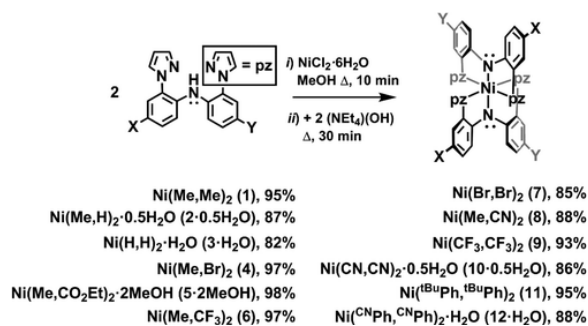
Scheme 1. Preparation of Ni(X,Y) 2 Complexes
