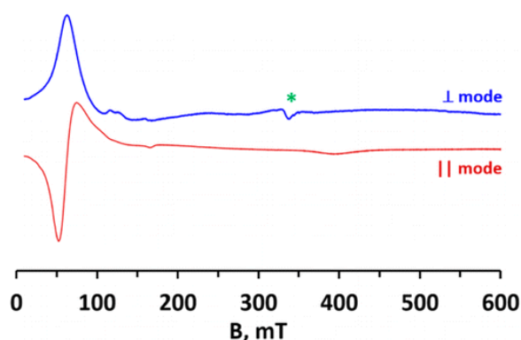
Figure 8. X-band EPR spectrum of (1) (BF 4 ) 2 ·0.5CH 2 Cl 2 in frozen (10 K) CH 2 Cl 2 acquired in both perpendicular (blue line) and parallel (red line) modes. The signal near 330 mT from a paramagnetic impurity in the sample chamber is demarcated with a green asterisk. Instrumental parameters: parallel mode, freq = 9.387 GHz; power = 10.0 mW, modulation 10 G; perpendicular mode, freq = 9.632 GHz, power = 2.0 mW, modulation 10 G.
